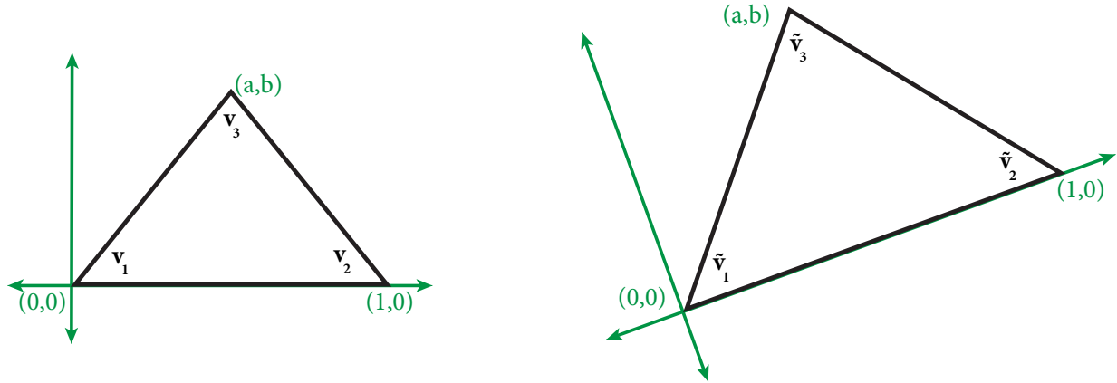
Figure 3.4: Warp mesh triangle before and after a similar transform. The local coordinate frame \{(\mathbf{v}_2 - \mathbf{v}_1), R_{90} \cdot (\mathbf{v}_2 - \mathbf{v}_1)\} attached to the triangle is shown in green.
