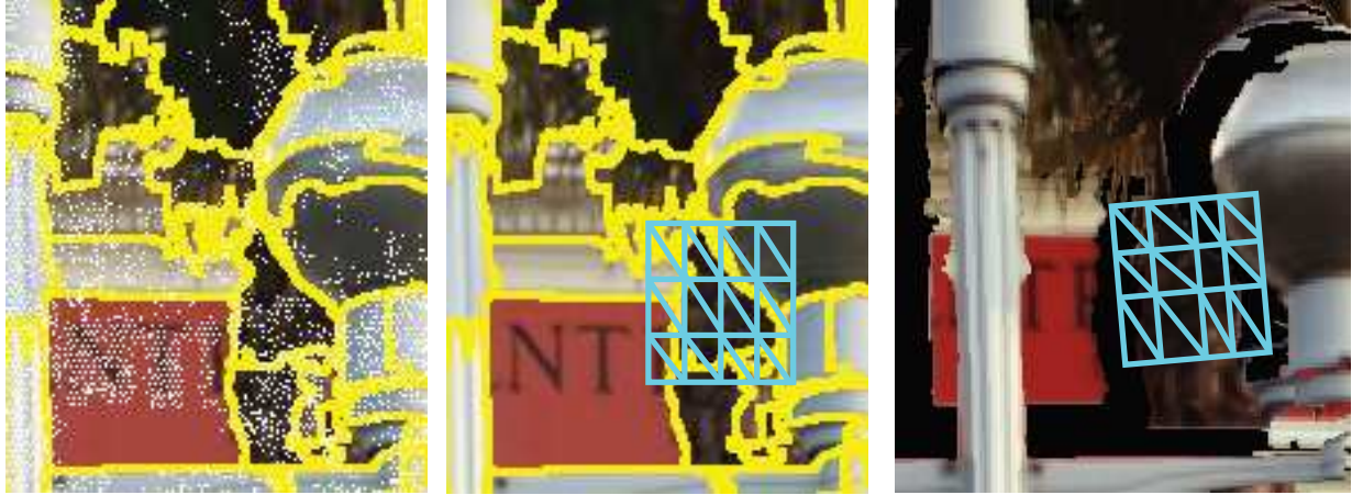
Figure 4.5: Left: Superpixel segmentation showing superpixels at multiple depths as well as depth samples contained inside each superpixel (shown as white dots). Middle: The regular grid which is used as warp mesh, overlaid over each superpixel. Right: Warped superpixels and grid for a novel view. Warping each superpixels independently preserves all silhouettes. Note how background superpixels slide under foreground.
