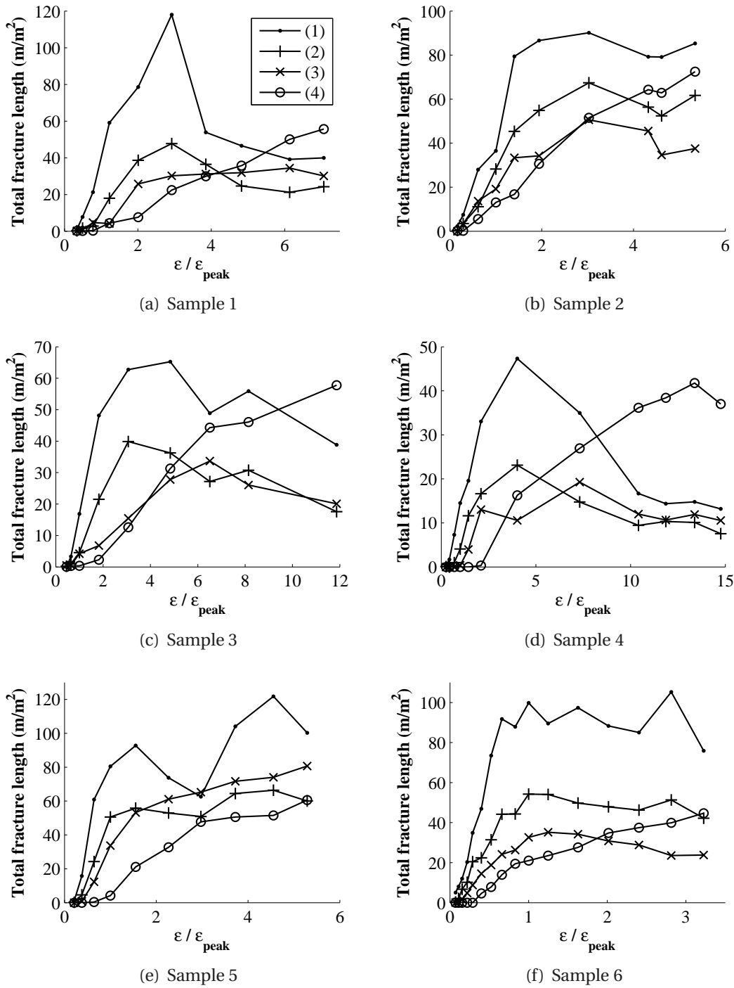
Figure 3.7: Visible fracture length per square meter of sample surface : (1) 3 \leq w < 5 \mu m , (2) 5 \leq w < 10 \mu m , (3) 10 \leq w < 50 \mu m , (4) w \geq 50 \mu m
