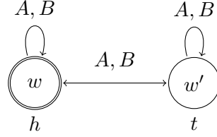
Figure 7.1: The epistemic model \mathcal{M} .
