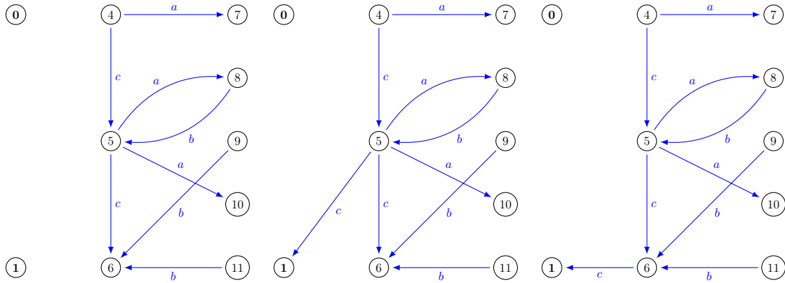
FIGURE 5.9 – La tuile A_{21}
