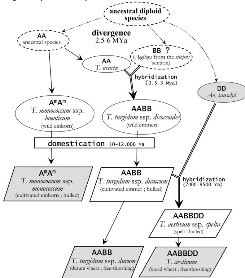
Figure 1.3: Schematic representation of the evolutionary history of wheat species ( Triticum and Aegilops ). Wild and domesticated species are represented in circles and squares, respectively.
