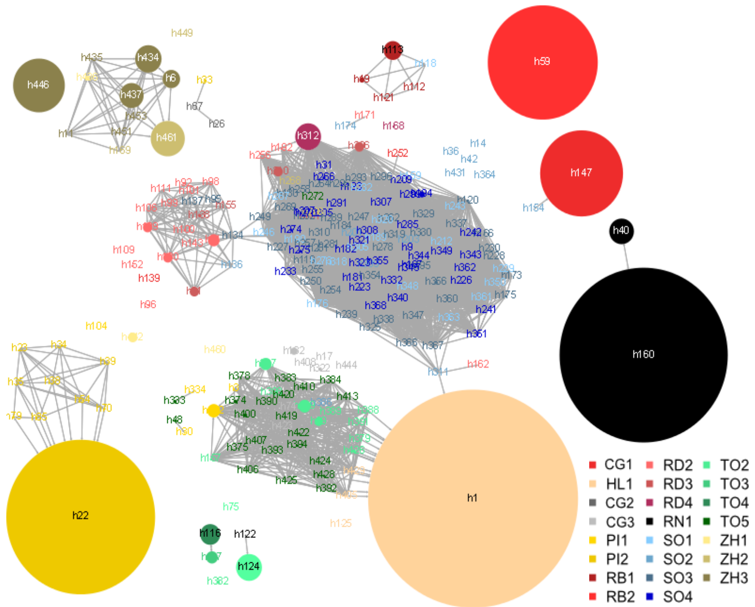
Figure 2.5. Overall haplotypic network of all the populations.
