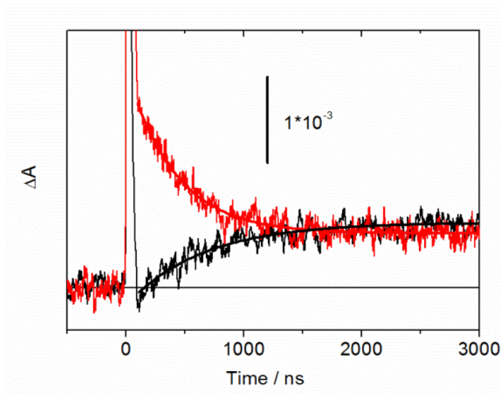
Figure 4.17: Kinetic traces at 510 nm (black) and 570 nm (red) with 100 \text{ mM } [\text{Ru}(\text{NH}_3)_6]^{3+} as electron acceptor in MeCN/H 2 O (50:50). The smooth lines represent best fits with monoexponential functions for t > 100 \text{ ns} .
