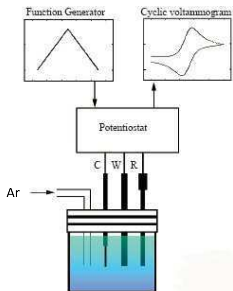
Figure 2.2: Typical experimental set up for measurement: R = Reference electrode: Ag/AgCl, W = working electrode: Glassy carbon, C= Counter electrode: Pt wire, Ar = Argon gas
