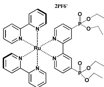
Figure 17 : Ru-Phosphonate, [\text{Ru}(\text{II})(\text{bpy})_2(4,4'-(\text{PO}_3\text{Et}_2)_2\text{bpy})] 2\text{PF}_6^-
