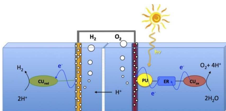
Figure 6.1: Photoelectrochemical cell
