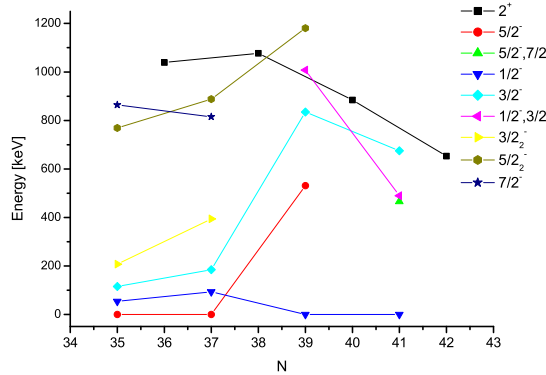
Figure 6.10: Systematics of negative-parity low-lying states in odd-Zn compared with the energy of the first 2^+ state in neighbouring energy level of the neighbouring even-Zn isotopes.
