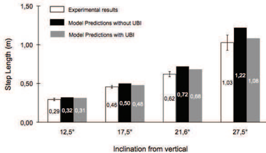
Figure 4.16: Step lengths for single step recovery scenarios from Hsiao-Wecksler and Robitnovitch (2007): experimental (white bars, averaged across subjects \pm one standard deviation) versus simulated (with and without UBI) results. The step timings are fixed in advance according to the reported values in the study.
