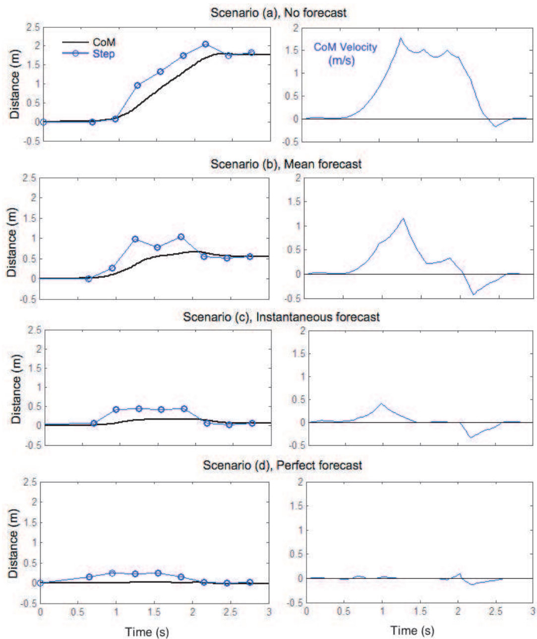
Figure 5.11: The predicted recovery behavior under the emergency braking scenario (c.f. Figure 5.9) with no or varying levels of disturbance forecasting. Time profiles of CoM position (left, black plot) and velocity (right) are plotted. The step positions are indicated with blue dots.
