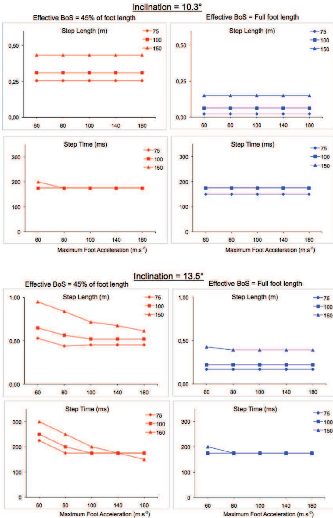
Figure 5.13: Optimized step lengths and timings against forward inclinations scenario for elderly from Hsiao-Weckslar and Robinovitch (2007) against maximum foot acceleration values (varied along x-axis) for 3 different reaction time values (75, 100 and 150 ms) and 2 different effective BoS lengths: (left red plots for reduced BoS vs. right blue plots for full BoS).
