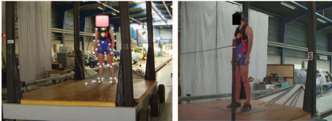
Figure 5.2: The two recovery tasks given to the subjects against the same level of disturbance; large available space (left) vs. limited space (right).
