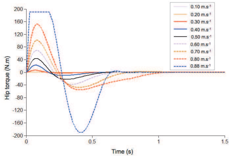
Figure 4.9: Time plots of resulting hip torque after the system is exposed to disturbances of increasing magnitudes till the limit of the combined ankle+hip strategies
