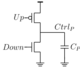
Figure 8.74 – Illustration of the structure of the charge pump. The voltage Ctrl_P of the delay line is driven by current injection of the capacitor C_P via the two transistors.
