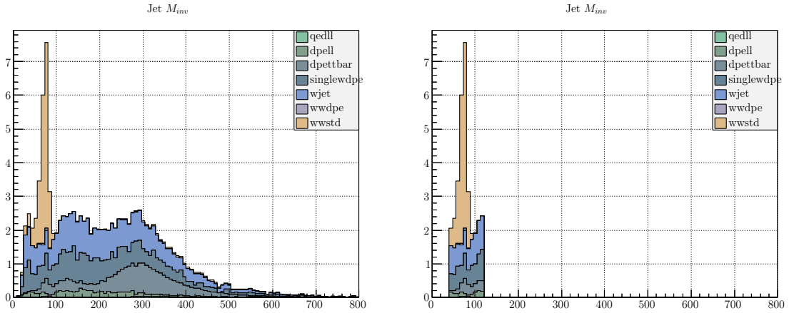
Figure 4.12 – Reconstructed dijet mass before (left) and after (right) the cut 40\text{GeV} \leq \text{dijetmass} \leq 120\text{GeV} . The cut selects the sharp dijet mass peak around the W mass for the signal (in orange) while removing background events having a dijet mass spread out.
