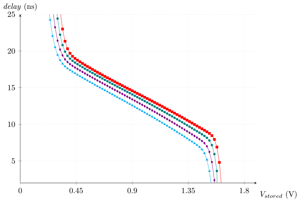
Figure 8.92 – Simulation of the delay of the comparator versus the stored voltage V_{store} on the switch, for the temperature T = 0^\circ C —▲—, T = 25^\circ C —◆—, T = 50^\circ C —●—, T = 75^\circ C —■—.
