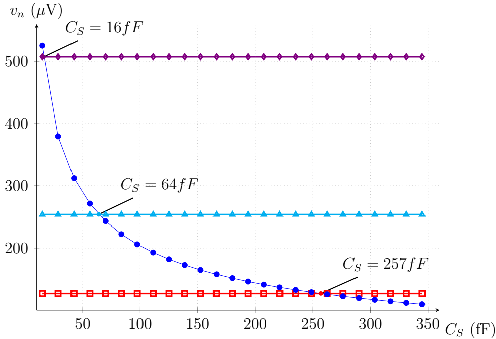
Figure 8.19 – Plot of the sampling noise value k_B T C ( - \bullet - ) as a function of the sampling capacitor. The quantization noise levels for 12- ( - \square - ), 11- ( - \blacktriangle - ) and 10-bits ( - \blacklozenge - ) are displayed and their intersection with the noise curve printed.
