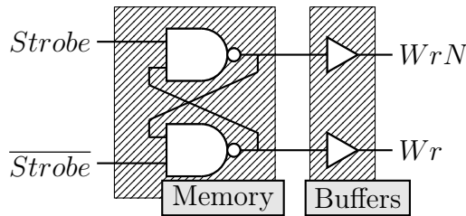
Figure 8.106 – Equivalent circuit in sampling mode ( Trig = 0 ).
