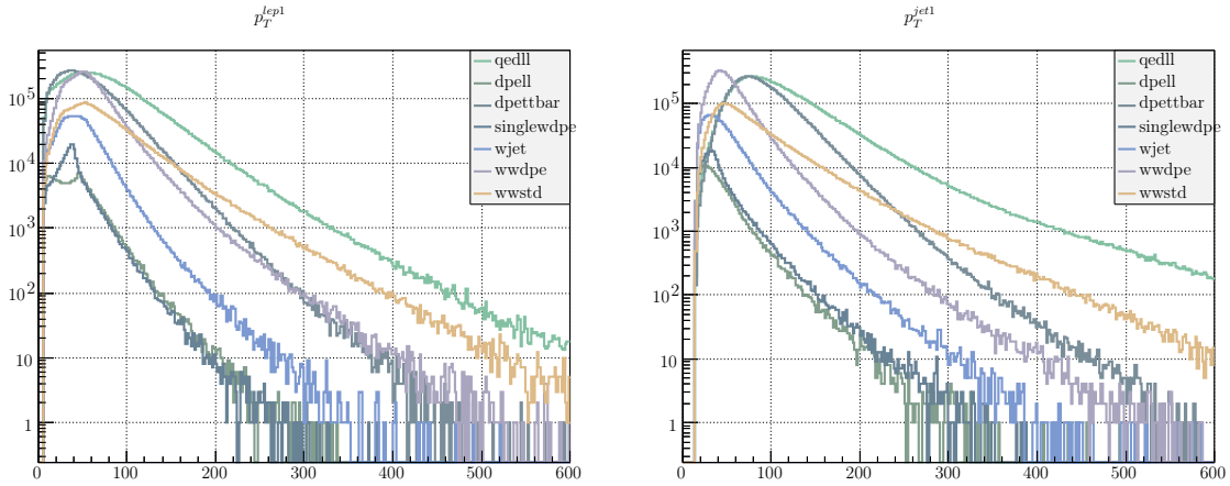
Figure 4.10 – Cumulated plot of the p_T of the leading jet and leading lepton for signal and backgrounds. In both cases the signal has a higher p_T lepton or jet.
