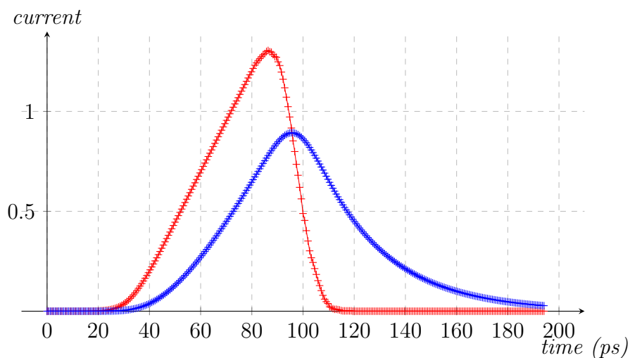
Figure 5.29 – Simulation of pulse shape degradation due to the anode frequency limitations. The current excitation of the anode is plotted in red ( -+ ) and the response of the anode is plotted in blue ( -+ ) for a cutoff frequency of 8GHz.
