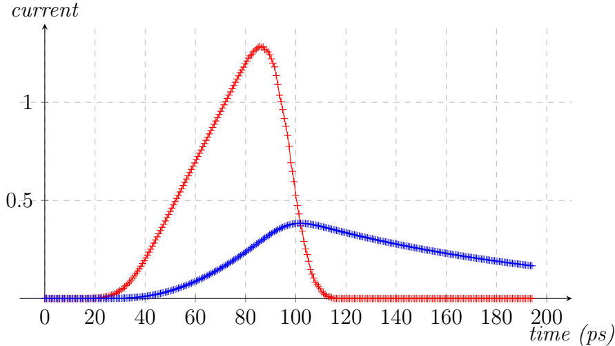
Figure 5.28 – Simulation of the pulse degradation due to the anode frequency limitation. The current excitation of the anode is plotted in red ( -\text{+} ) and the response of the anode is plotted in blue ( -\text{+} ) for a cutoff frequency of 2 GHz.
