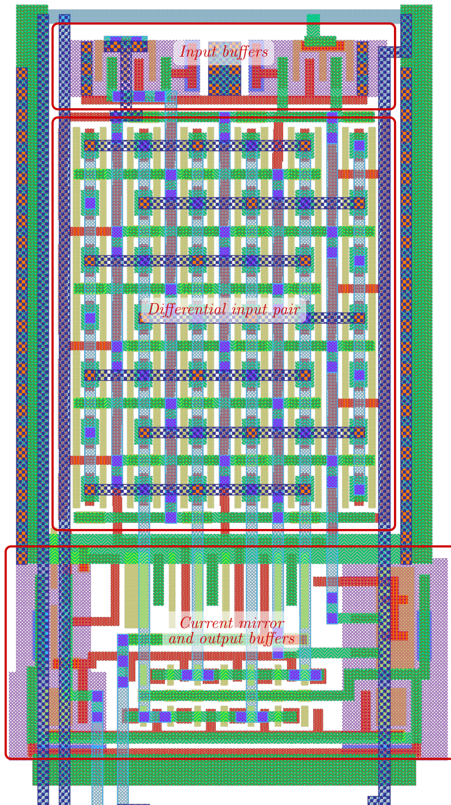
Figure 8.93 – Layout of the comparator.
