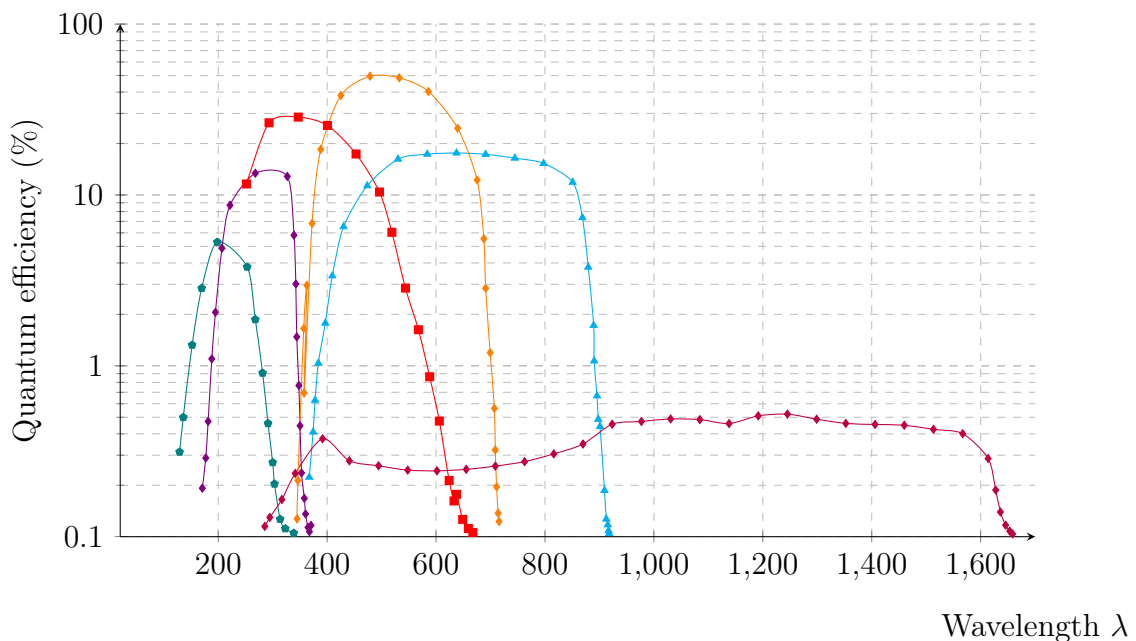
Figure 5.10 – Quantum efficiency versus wavelength of various photocathodes: Cs-Te ( \bullet ), GaN ( \blacklozenge ), SuperBialkali ( \blacksquare ), GaAsP ( \blacktriangleleft ), GaAs ( \blacklozenge ), InP ( \blacklozenge ). Quantum efficiency is the ratio of photoelectrons emitted from the photocathode to the number of incident photons, expressed in percent.
