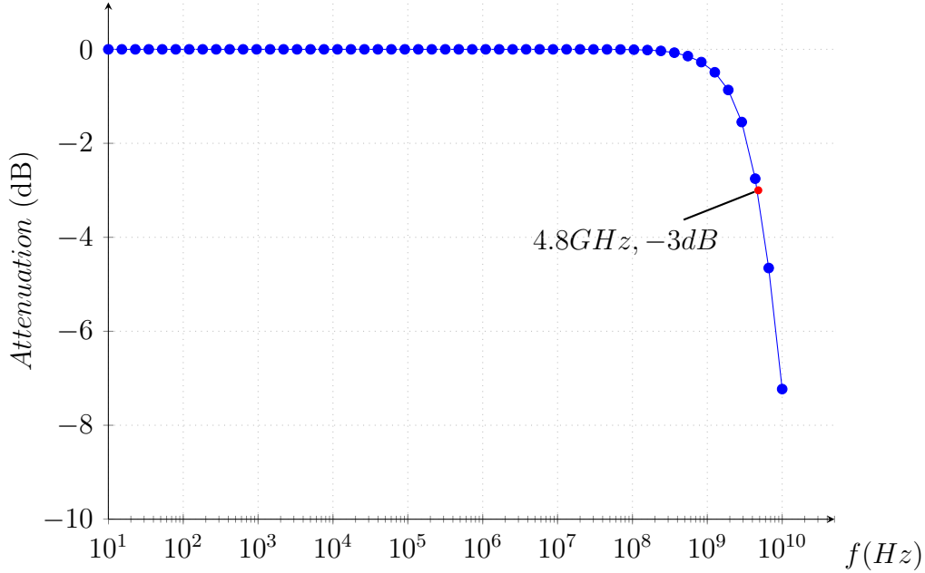
Figure 8.28 – Simulation of the minimum bandwidth of the sampling cell versus the frequency ( W = 2 \mu m , C_S = 35 \text{ fF} ).
