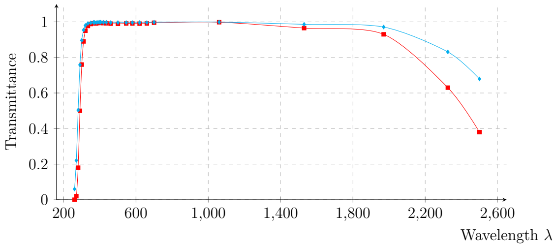
Figure 5.5 – Transmission of the NF-K5 glass from Schott [11] for a thickness of 10mm ( \text{---}\blacklozenge\text{---} ) and 25mm ( \text{---}\blacksquare\text{---} ).
