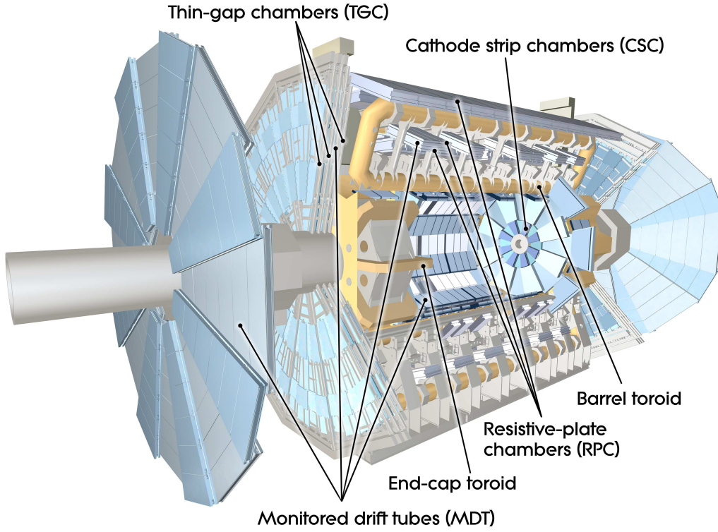
Figure 2.6 – Cut-away view of the ATLAS muon system.
