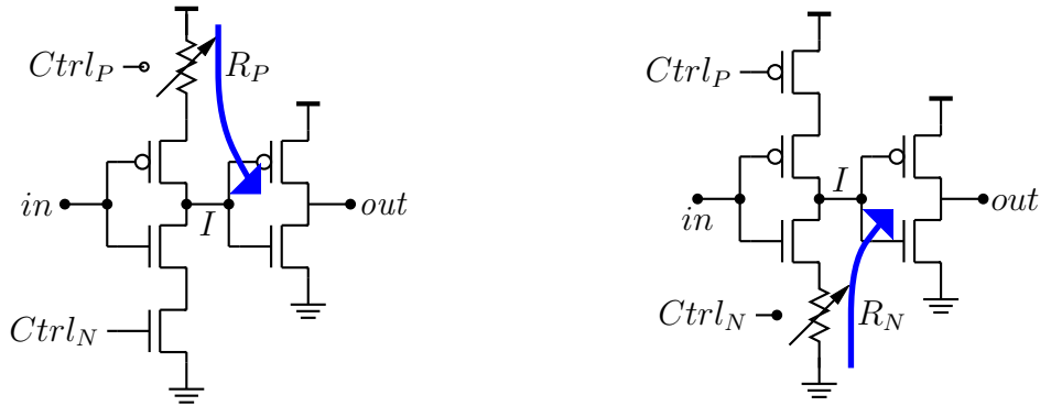
(b) Current paths during rising edge.
