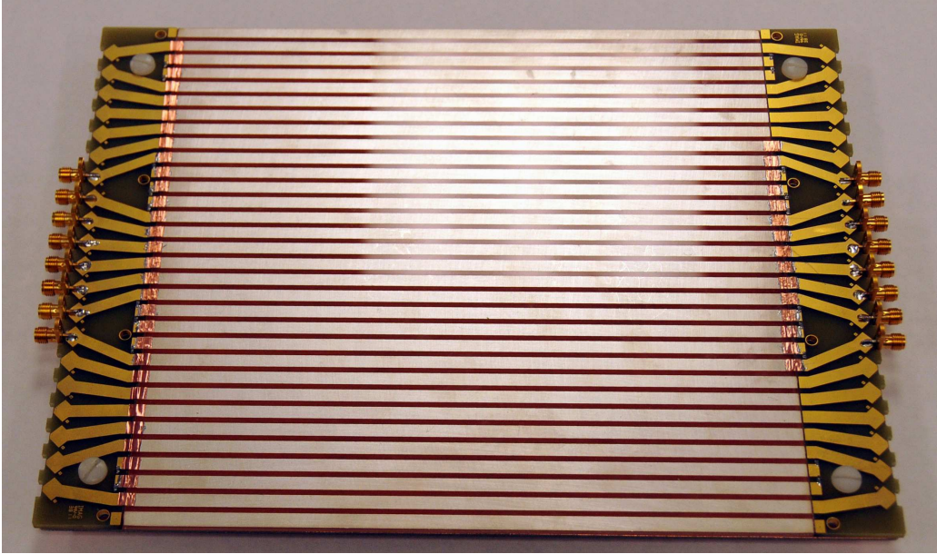
Figure 5.21 – Photograph of the 30-strip anodes array used to collect and transmit current pulses from the 8 inch LAPPD photo-detector. The anode array has been connected to two side cards (on the picture) used for characterization of its radio-frequency properties.
