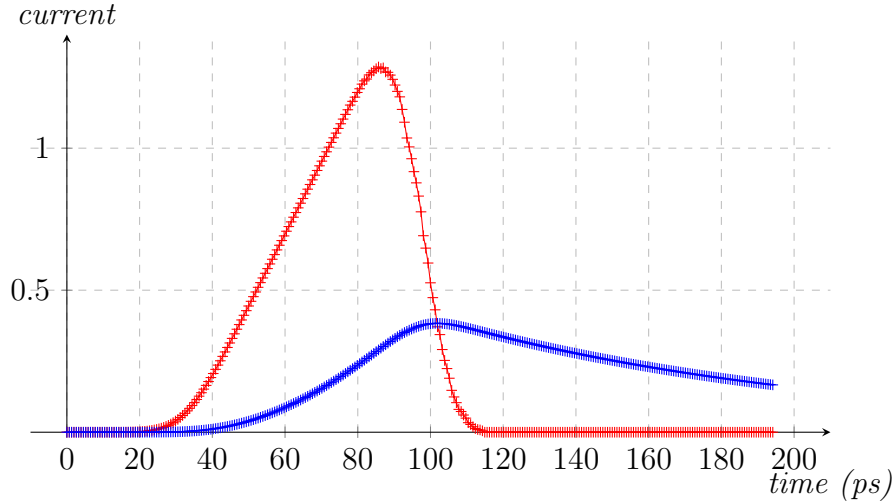
Figure 5.28 – Simulation of the pulse degradation due to the anode frequency limitation. The current excitation of the anode is plotted in red ( + ) and the response of the anode is plotted in blue ( + ) for a cutoff frequency of 2 GHz.
