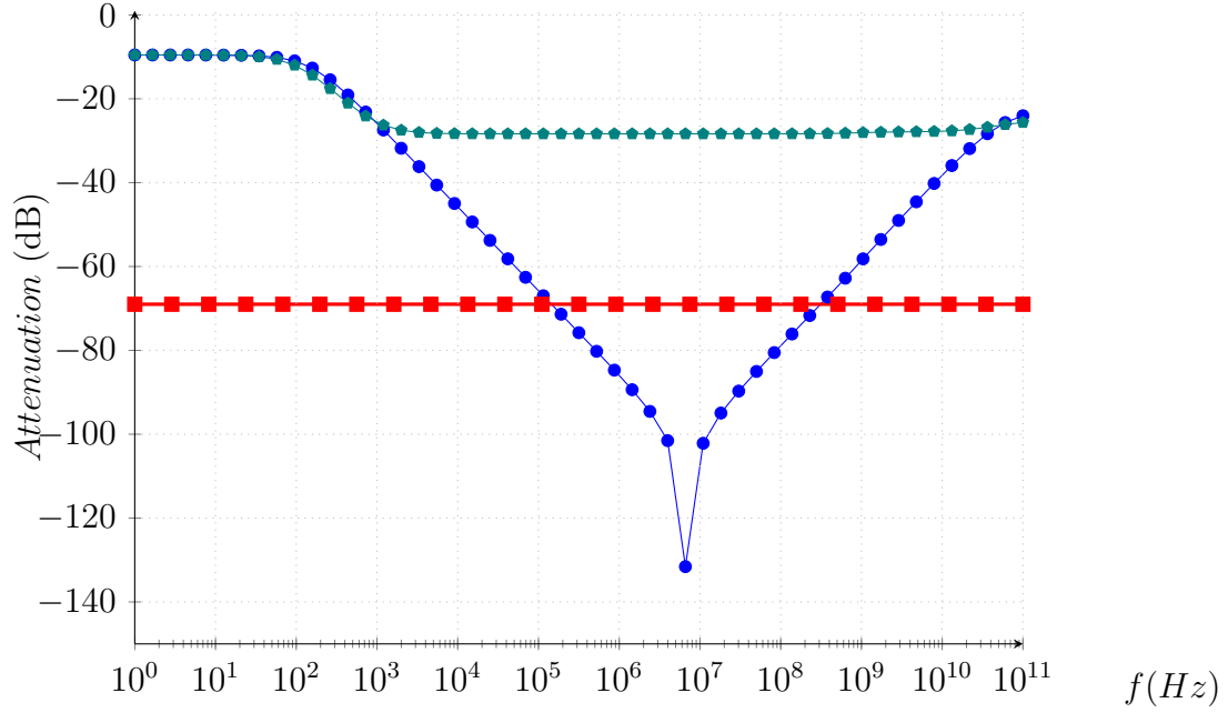
Figure 8.32 – AC simulation of the coupling magnitude from the input signal V_{in} to the sampling capacitor, in dB. The simulation was done for coupling with —●— and without —●— considering parasitic effect of the layout design. The kTC noise —■— of the sampling cell is also printed for comparison.
