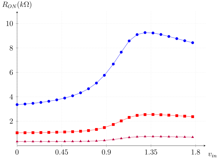
Figure 8.27 – Simulation of the ON resistance of the switch as a function of the input voltage v_{in} for three different switch size: 500nm \bullet , 1.6μm \blacksquare and 5μm \blacktriangle . The switch PMOS and NMOS sizes are equal.
