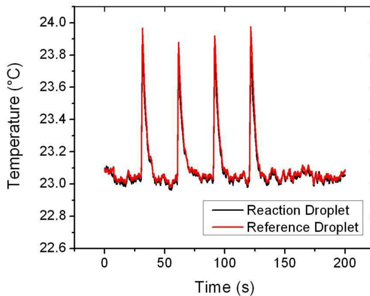
Figure 5.5 Thermal camera measurements of the temperature perturbation profile in 10 \mu\text{l} droplets resulting from a 30 dBm SAW excitation pulse train with a period of 30s and a duty cycle of 1/30 (1 sec on and 29 sec off).
