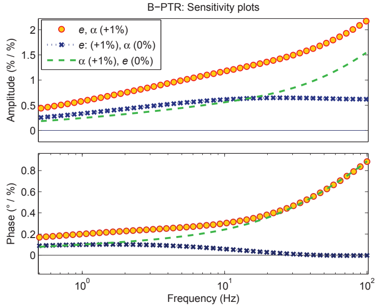
Figure 3.4: Simulated plots of frequency dependent amplitude and phase of a typical liquid sample ( \alpha_1 = 1.48 \times 10^{-7} \text{m}^2 \text{s}^{-1} , e_1 = 650 \text{Jm}^{-2} \text{K}^{-1} \text{s}^{-1/2} , d = 50 \mu\text{m} ) showing the percentile change in amplitude (upper plot) and phase (lower plot) with +1% change in \alpha_1 and e_1 , (circles); +1% change in e_1 keeping 0% change in \alpha_1 (dotted line with cross) and +1% change in \alpha_1 keeping 0% change in e_1 (dashed line).
