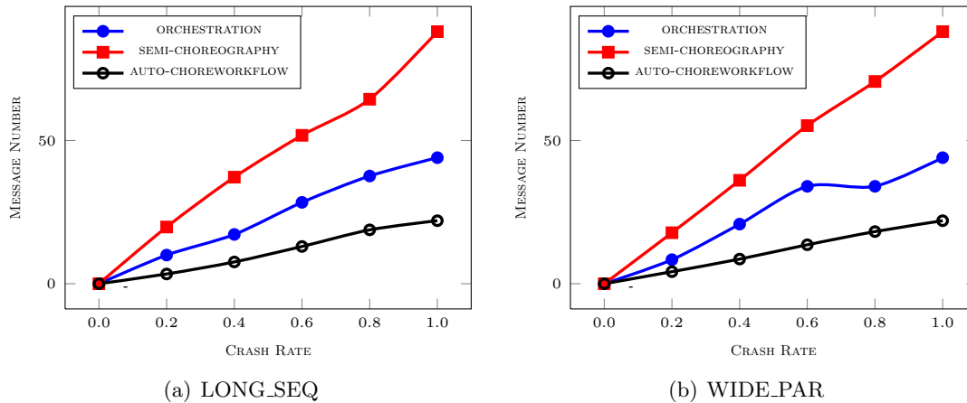
Figure 4.10: The Number of Additional Messages for Different Models
