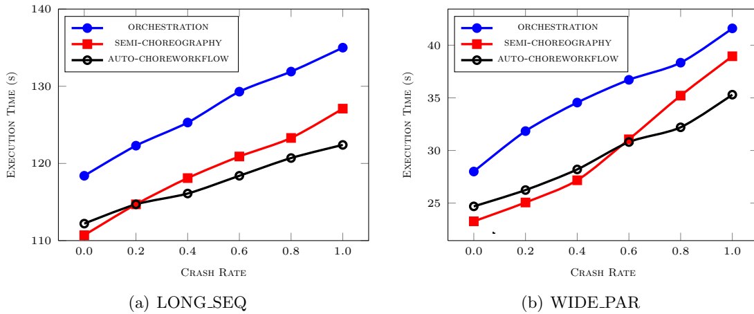
Figure 4.11: The Overall Execution Time (Including Adaptation) for Different Models
