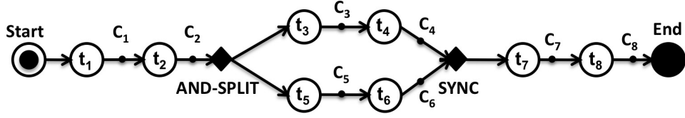
Figure 5.5: Experimental Workflow
