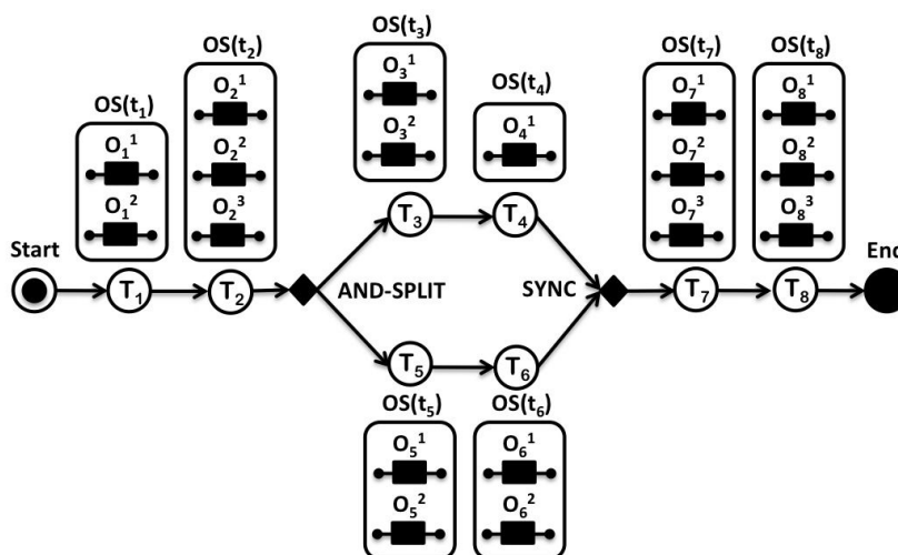
Figure 3.4: Offer Sets
