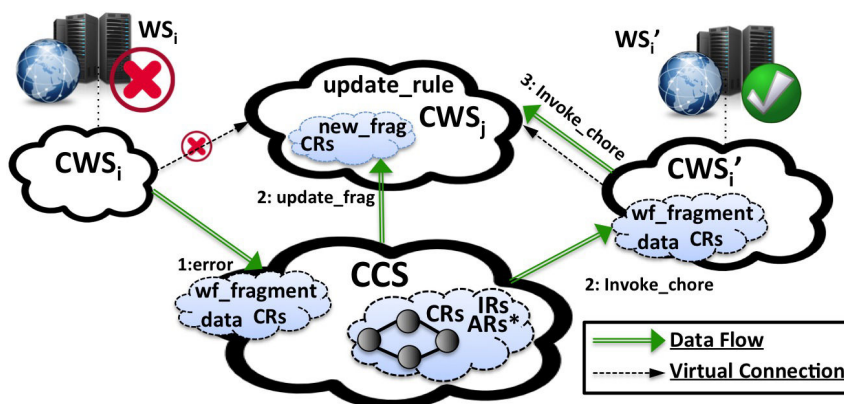
Figure 3.20: Semi-Choreography Model: Binding-Level Adaptation
