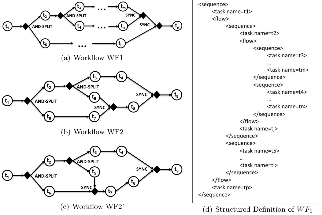
Figure 2.1: Structured Workflow Definition
