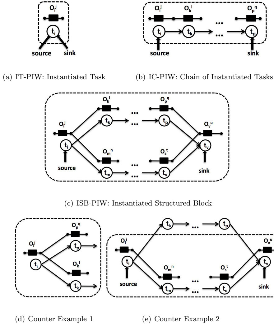
Figure 3.5: Partially Instantiated Workflow (PIW)
