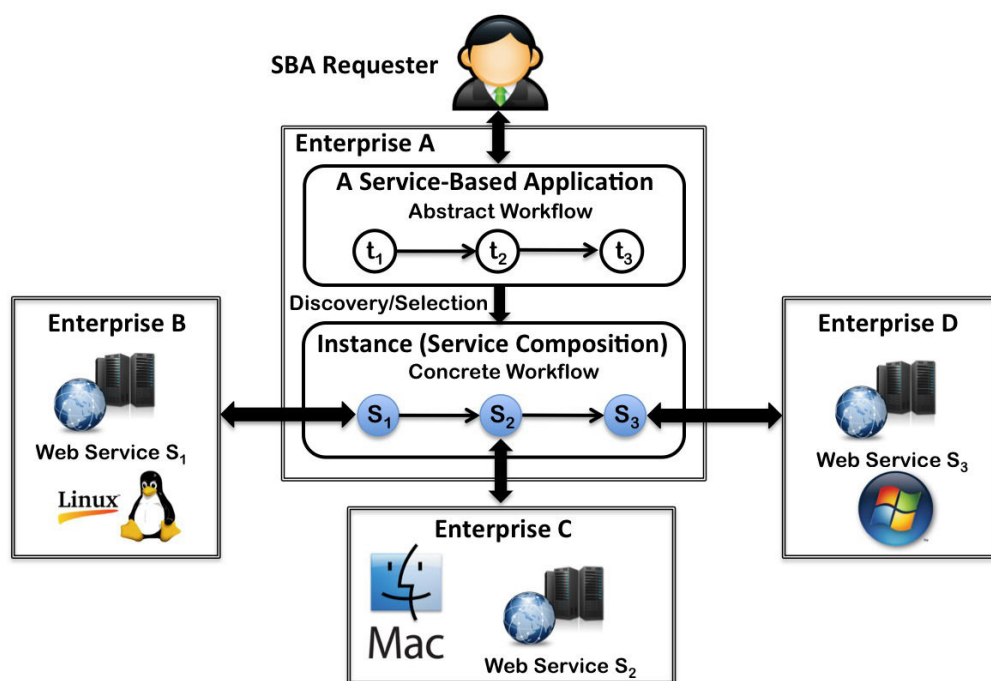
Figure 1.1: Service-Based Application
