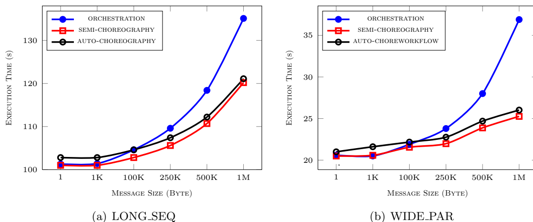
Figure 4.9: The Execution Time for Different Models
