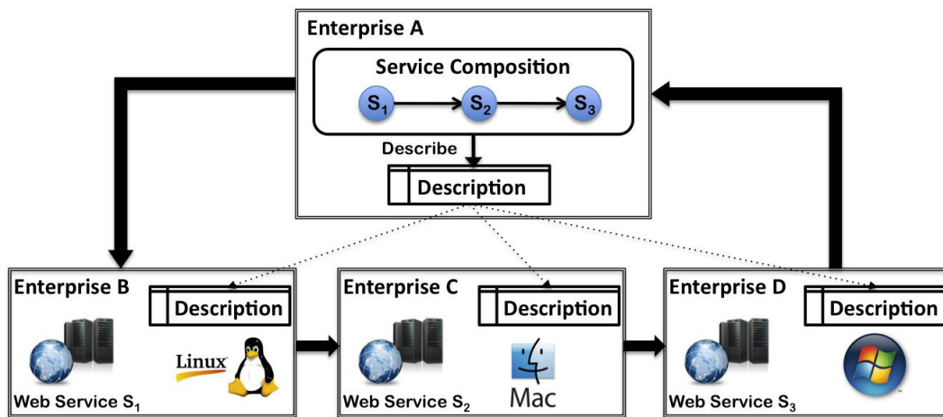
Figure 1.8: Web Service Choreography Model
