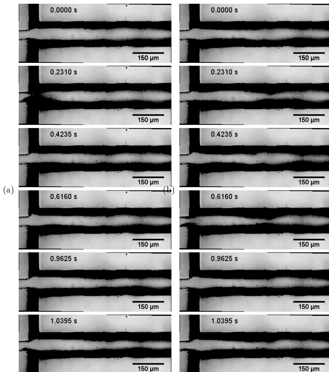
Figure 6.7.: Interfacial evolution between two miscible liquids under an AC electric field of 3000\text{V/cm} and a frequency of (a) 1\text{Hz} and (b) 2\text{Hz} . The dark liquid is a solution of 0.01\text{M} Rhodamine B in DI water and the clear liquid is an aqueous electrolyte (see text for details) with a conductivity of 1500\mu\text{S/cm} . Both liquids have an additional imposed flow rate of 500\text{nl/min} .
