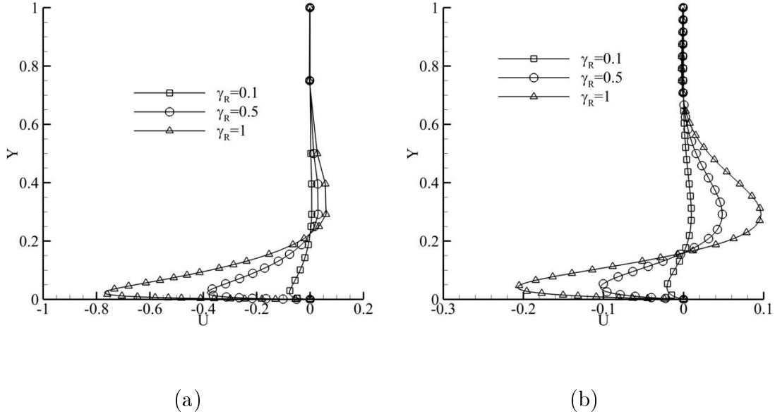
Figure 3.5.: Velocity distribution over the film thickness with different values of Electro-osmotic number, \gamma_R for \beta = 5 , Z_R = 0 , Wo = 10 at \Theta = \pi/2 with (a) De = 0.01 and (b) De = 0.1 .
