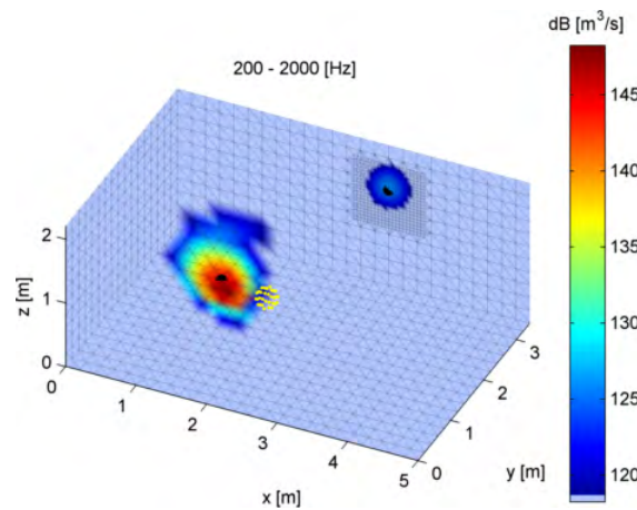
Figure 4.12: Volume velocity map integrated over the 200-2000 Hz frequency band using the iterative weighted approach. The results are for the model with local refinement and the second iteration. Notice that the dynamic range is set to 30 dB.
