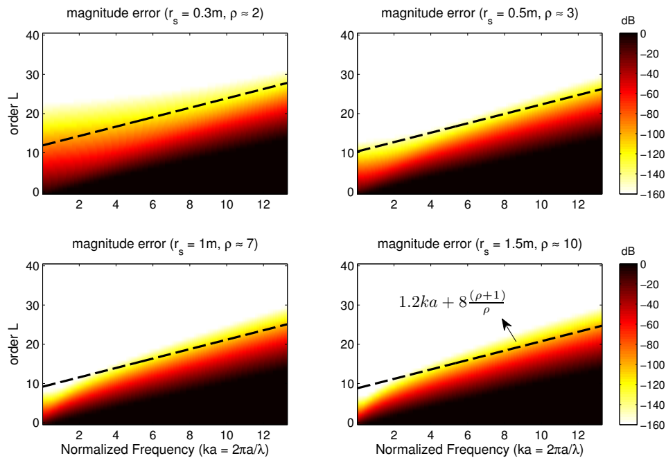
Figure 2.11: Averaged magnitude error as a function of normalized frequency ( ka ) for the rigid sphere configuration. The results are given for different distances ( r_s ) from the center of the array. The figure also shows the regression line from equation (2.61) used to bound the number of orders to be evaluated.
