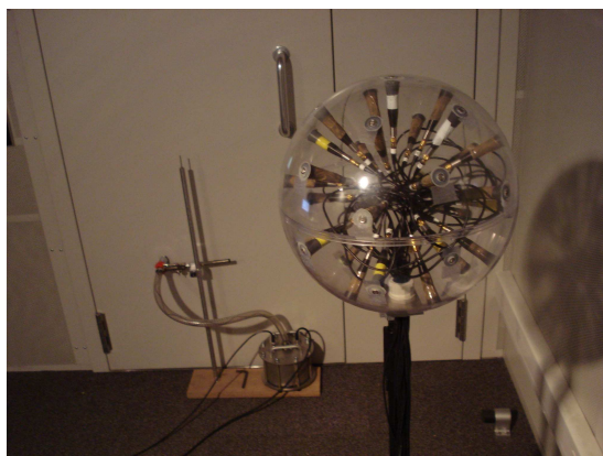
Figure 5.6: Measurement set-up.
