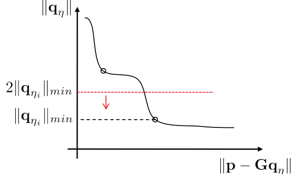
Figure 3.5: Schematic L-curve for the case with multiple local maxima.
