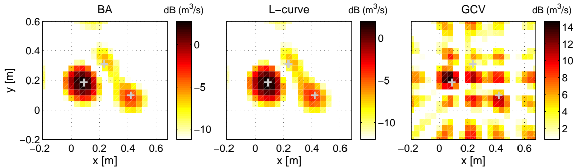
Figure 3.23: Reconstructed source field (volume velocity) at 945 Hz corresponding to each regularization criterion. A dynamic range of 15 dB is used for all.
