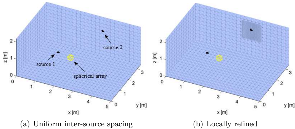
Figure 4.10: Models used to study the influence of the homogeneity of equivalent sources distribution. (a) model with a uniform inter-source spacing of 0.2 m; (b) Model with a local refinement (inter-source spacing 0.05 m) around source 2.
