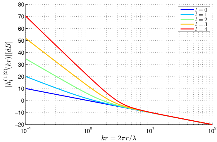
Figure B.2: Magnitude of the spherical Hankel functions |h_l^{(1/2)}(kr)| . Notice that higher-order components decay quickly with increasing kr . These functions represent traveling wave type solutions of the Helmholtz equation.
