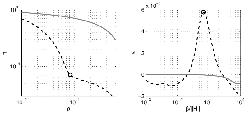
Figure 3.8: L-curve (left) and its curvature (right) at 800 Hz (dashed black) and 1400 Hz (solid gray).
