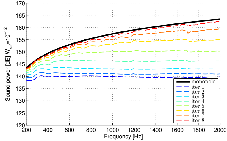
Figure 4.15: Identified acoustic power as a function of the frequency for the model with a local refinement area. The results are for the source 2, which is located on the refined region.
