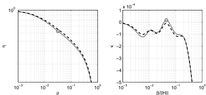
Figure 3.12: L-curve (left) and its curvature (right) at 1295Hz (solid gray) and 1300Hz (dashed black).
