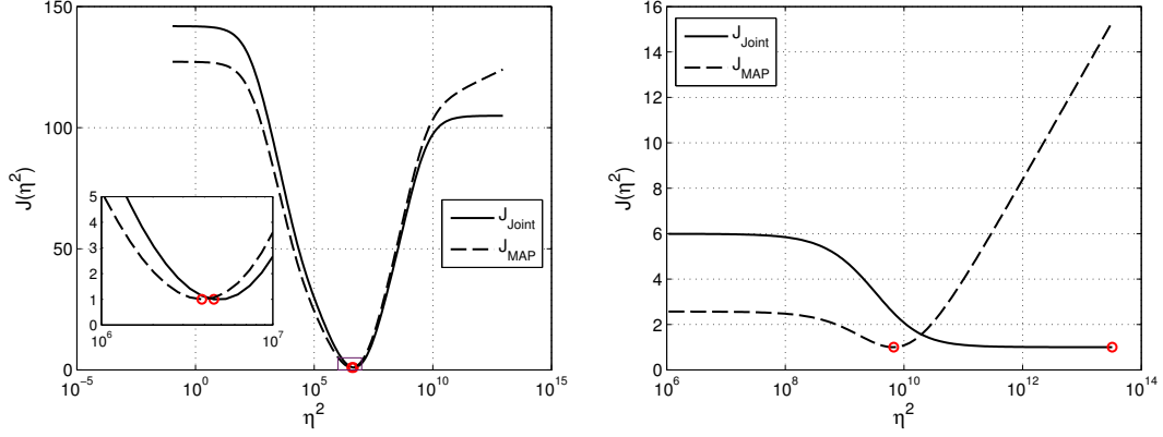
Figure 3.2: In most practical situations \hat{\eta}_{\text{Joint}}^2 and \hat{\eta}_{\text{MAP}}^2 are found nearly equal (see left panel). One exception is when the SNR is so poor that \mathbf{J}_{\text{Joint}} tends to see only noise, thus rejecting its minimum to infinity and returning an unbounded value of the regularization parameter. Such a situation is forbidden by \mathbf{J}_{\text{MAP}} which, by construction, advantageously forces a finite value of \eta^2 (see right panel).
