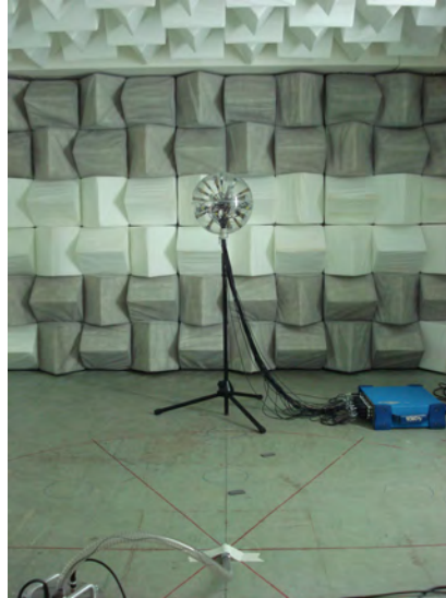
Figure 5.11: Measurement set-up.
