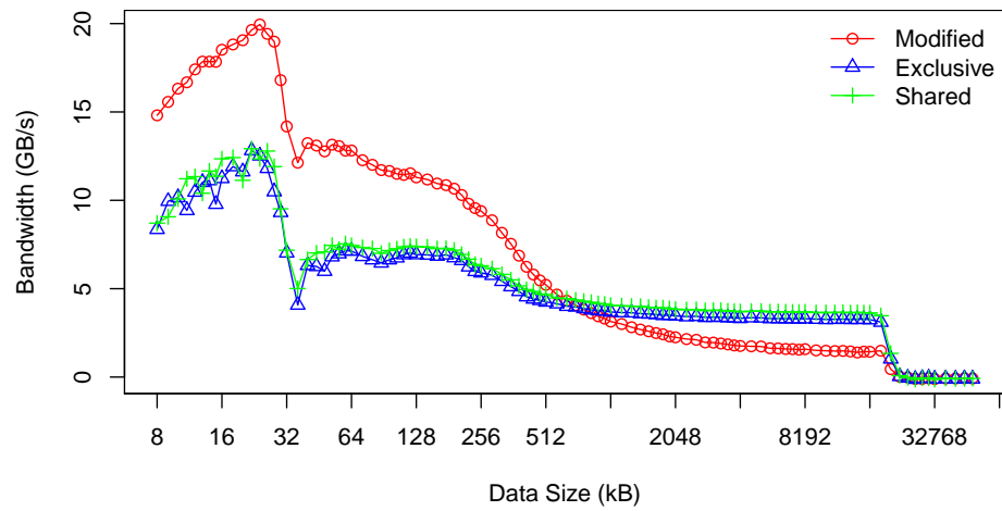
Figure 2.9: Cost of an RFO message depending on the state of the cache line involved.
