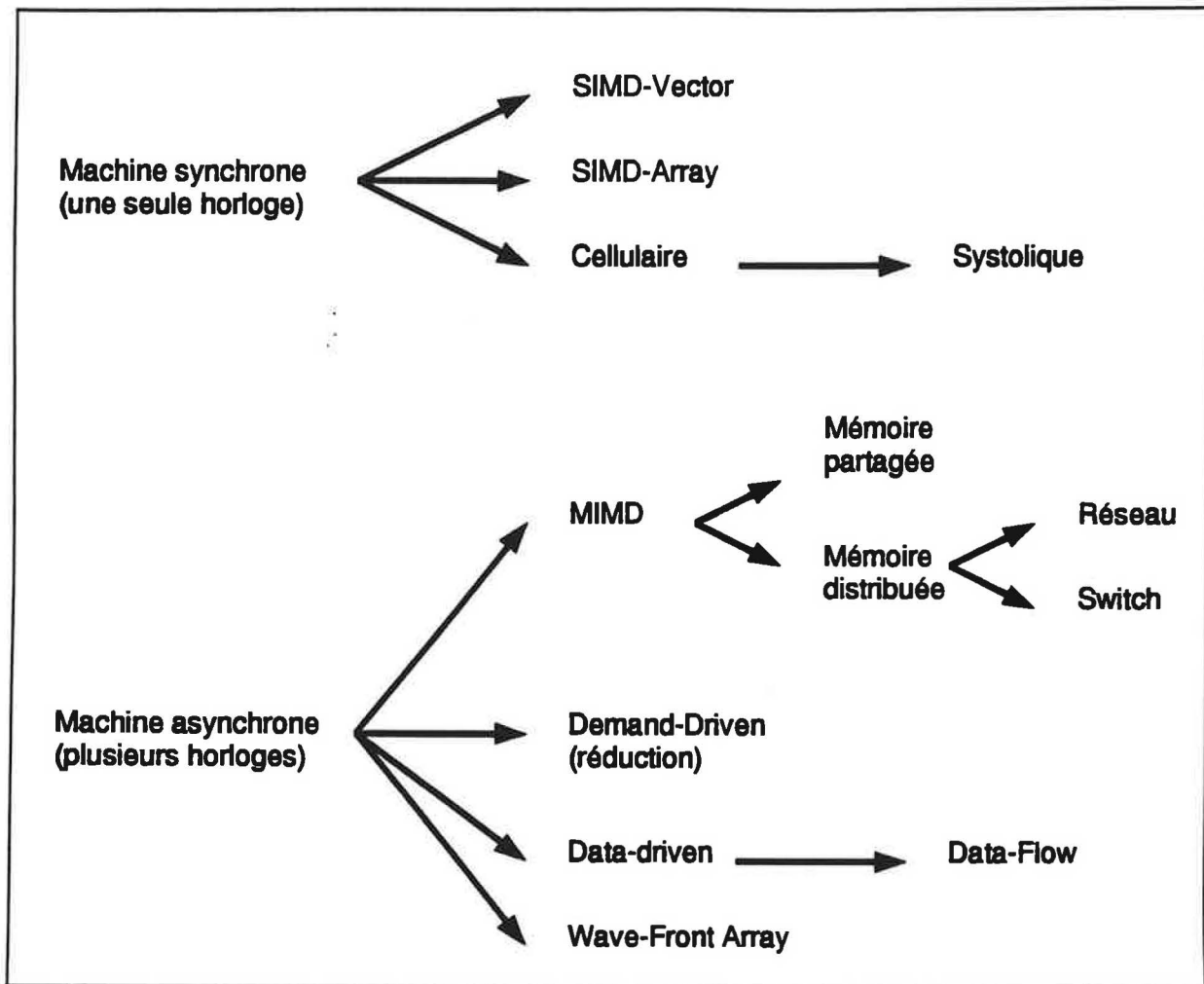
Figure 24 La classification de MIMESIS
