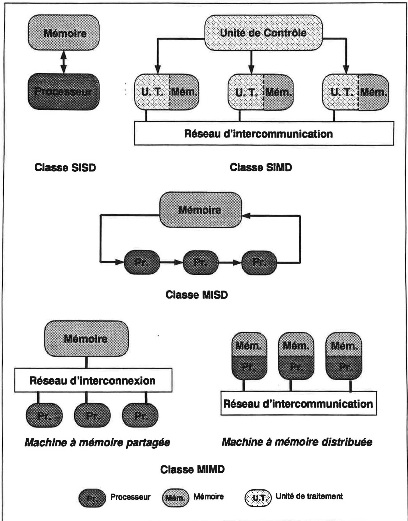
Figure 22 La classification de Flynn
