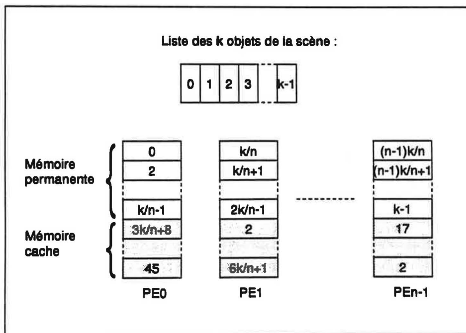
Figure 53 Organisation de la mémoire
