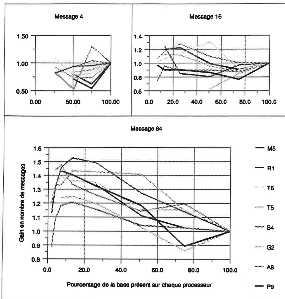
Figure 84 Gain en messages
