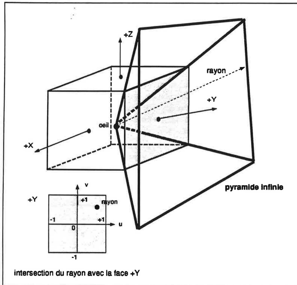
Figure 20 Le cube de direction
