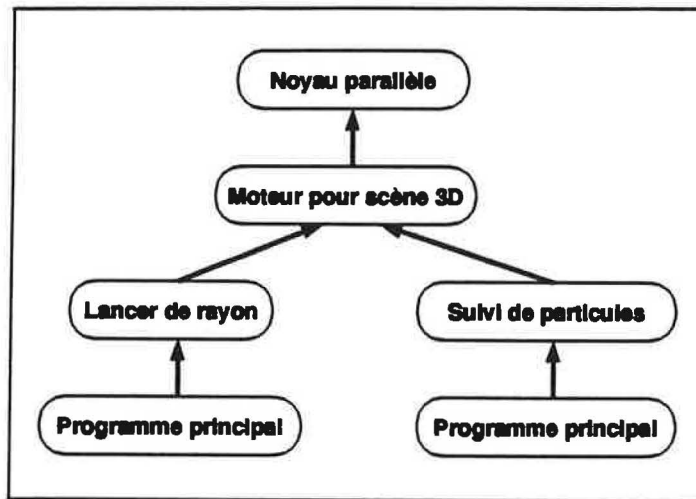
Figure 103 Architecture du code
