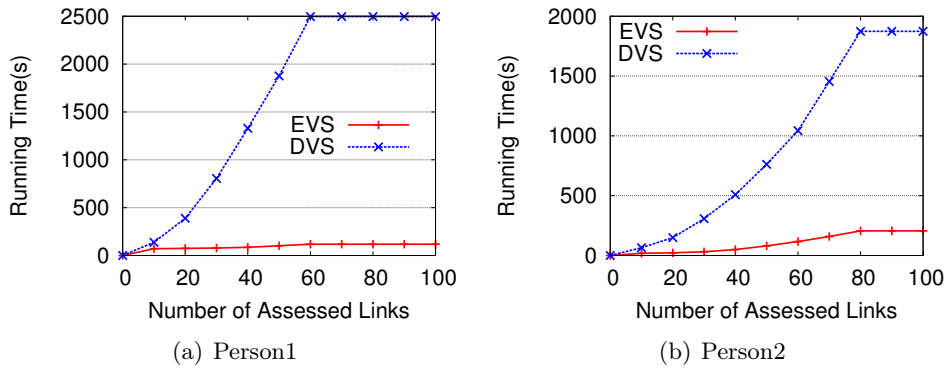
Figure 8.18: Running Time of Person1 and Person2
