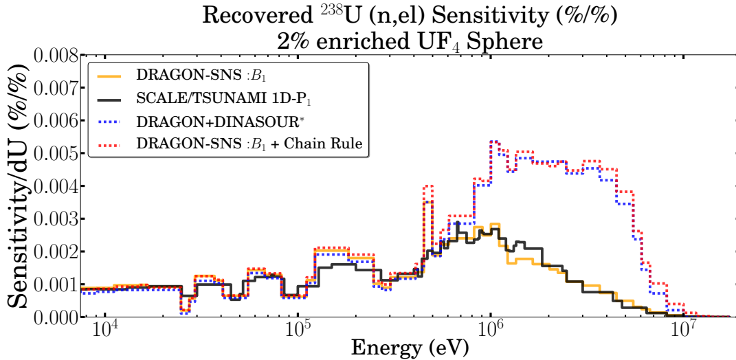
Figure 4.12: Comparison of the k_{eff} ^{238}\text{U} (n,el) sensitivity profiles for the \text{UF}_4 sphere. DRAGON-SNS: B_1 solution obtained using the ENDF B/VI (orange curve). SCALE/TSUNAMI-1D P_1 solution obtained using the ENDF B/VI evaluation (black curve). DRAGON+DINASOUR* results supplied by McMaster University using our input model and ENDF B/VII evaluation (dotted blue curve). DRAGON-SNS: B_1 + Chain rule obtained by applying the chain rule to the SNS: computed sensitivity (dotted red curve). Note the good comparison between DRAGON-SNS: B_1 with the reference solution SCALE/TSUNAMI-1D P_1 and the poorly computed sensitivity resulting from applying the chain rule.
