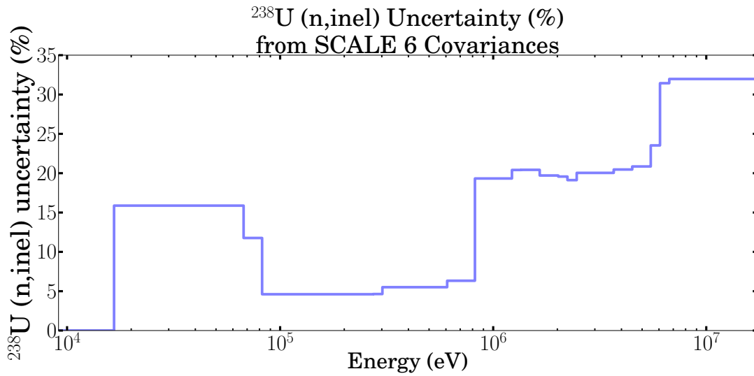
Figure 3.9: ^{238}\text{U} (n,inel) uncertainty(%) from SCALE 6 Covariances
