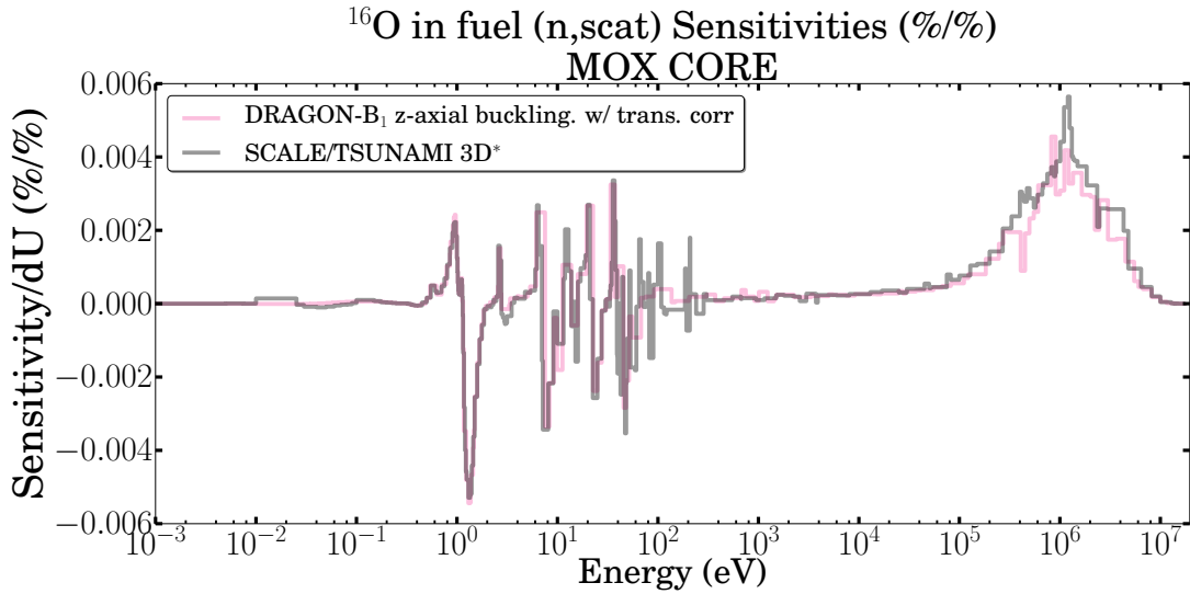
Figure 4.27: MOX core with light water reflector: ^{16}\text{O} (n,scat) sensitivity profile (\%/)/du *SCALE/TSUNAMI 3D P_5 results supplied by the IRSN[107] Note the good comparison of DRAGON- B_1 results with SCALE/TSUANMI 3D results for ^{16}\text{O} (n,scat) in the fuel where the buckling approximation is valid.
