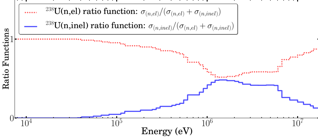
^{238}\text{U}(n,\text{el}) and ^{238}\text{U}(n,\text{inel}) ratio functions (no units) from JEFF 3.1
