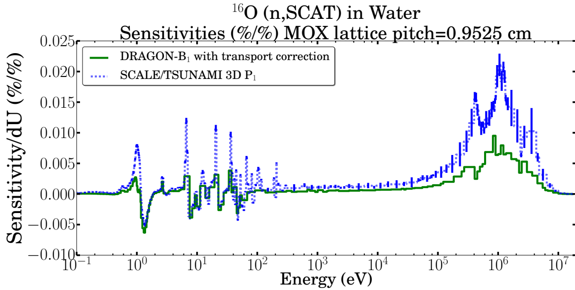
Figure 4.17: Comparison of ^{16}\text{O}(n,\text{scat}) in \text{H}_2\text{O} sensitivity profiles for MOX lattice at pitch=0.9525 cm. DRAGON B 1 with transport correction sensitivity profile (green). SCALE6/TSUNAMI-3D P 1 sensitivity profile (blue). Note the poor comparison between the two profiles arising from anisotropic effects.
