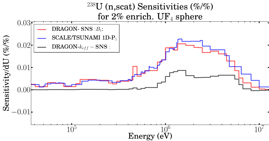
Figure 4.4: Comparison of ^{238}\text{U} (n,SCAT) sensitivity for the \text{UF}_4 sphere.
