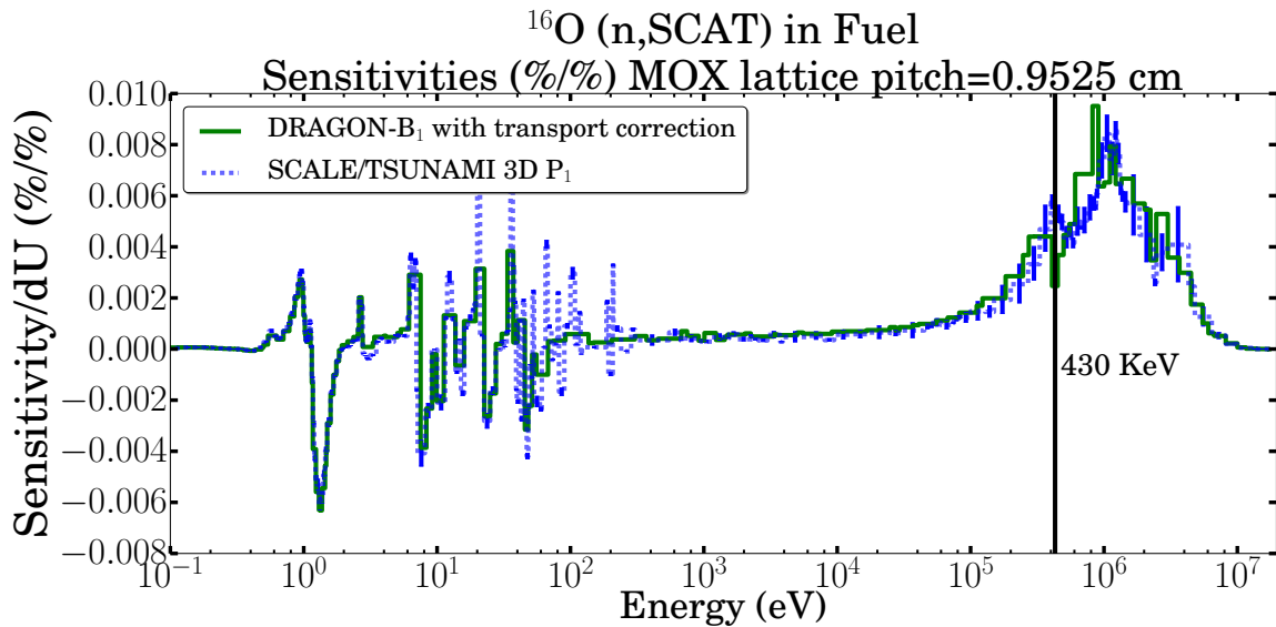
Figure 4.18: Comparison of ^{16}\text{O}(n,\text{scat}) in the fuel sensitivity profile for MOX lattice at pitch=0.9525 cm. DRAGON B 1 with transport correction (green). SCALE6/TSUNAMI-3D P 1 (blue). Note the effect of the resonance at 430 keV.
