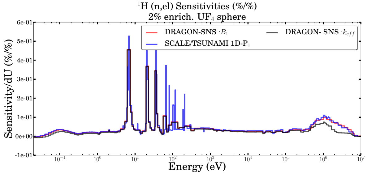
Figure 4.1: Comparison of ^1\text{H}(n,\text{el}) sensitivity for the \text{UF}_4 sphere. Note the differences at high energy between the gray curve and the two other curves, that result from streaming effects that are not captured by the DRAGON- k_{eff} (DR-K) approach.
