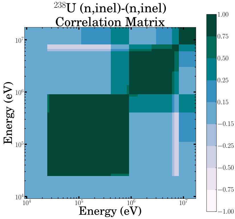
Figure 3.8: ^{238}\text{U} (n,inel)-(n,inel) correlation matrix from SCALE 6 Covariances
