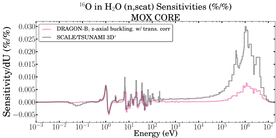
Figure 4.28: MOX core with light water reflector: ^{16}\text{O} (n,scat) in \text{H}_2\text{O} sensitivity profile (\%/)/du . *SCALE/TSUNAMI 3D P_5 results supplied by the IRSN[107] Note the discrepancy between the DR- B_1 and the S5- P_5 results throughout the spectrum due to the inadequacy of the buckling approximation in the light water reflector.
