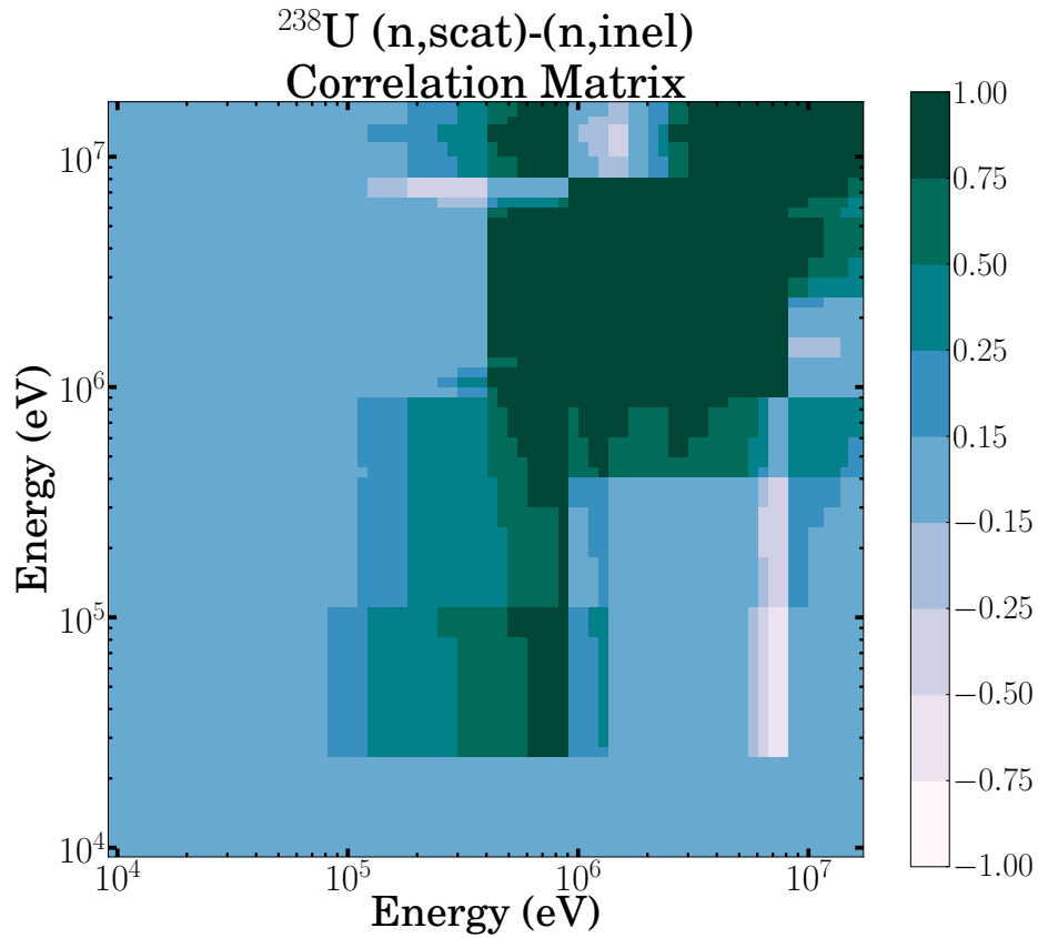
Figure 3.10: ^{238}\text{U}(\text{n,SCAT})-(\text{n,inel}) correlation matrix for groups 1-45 of the WIMS 172-group library. Constructed from SCALE 6 covariances and JEFF 3.1 cross section values.
