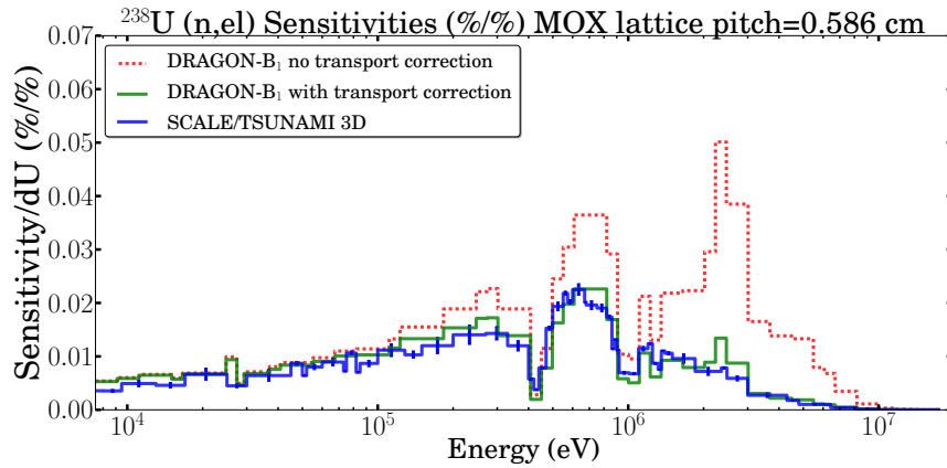
Figure 4.14: Comparison of ^{238}\text{U} (n,el) sensitivity for MOX lattice at pitch=0.586 cm.
