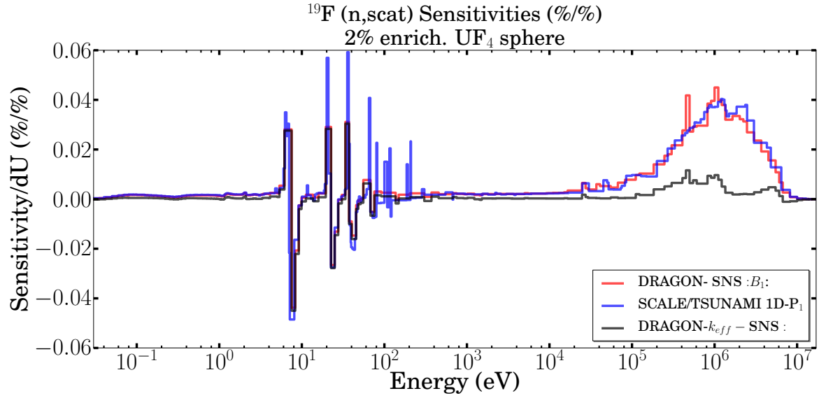
Figure 4.3: Comparison of ^{19}\text{F} (n,SCAT) sensitivity for the \text{UF}_4 sphere.
