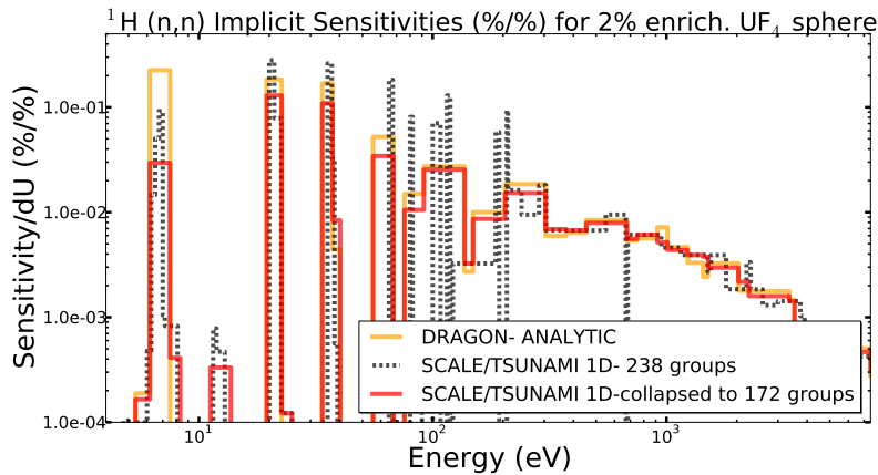
Figure 4.7: Negative component of the ^1\text{H} (n,scat) implicit sensitivity in the resonance region. One SHI : and the analytical approximation (orange curve); 238-group SCALE/TSUNAMI 1D implicit sensitivity profile (black dotted); SCALE/TSUNAMI-1D implicit sensitivity collapsed to the 172 group WIMS energy grid.
