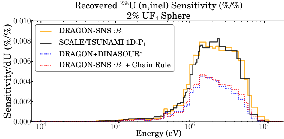
Figure 4.11: Comparison of the k_{eff} ^{238}\text{U} (n,inel) sensitivity profiles for the \text{UF}_4 sphere. DRAGON-SNS: B_1 solution obtained using the ENDF B/VI (orange curve). SCALE/TSUNAMI-1D P_1 solution obtained using the ENDF B/VI evaluation (black curve). DRAGON+DINASOUR* results supplied by McMaster University using our input model and ENDF B/VII evaluation (dotted blue curve). DRAGON-SNS: B_1 + Chain rule obtained by applying the chain rule to the SNS: computed sensitivity (dotted black curve). Note the good comparison between DRAGON-SNS: B_1 with the reference solution SCALE/TSUNAMI-1D P_1 and the poorly computed sensitivity resulting from applying the chain rule.
