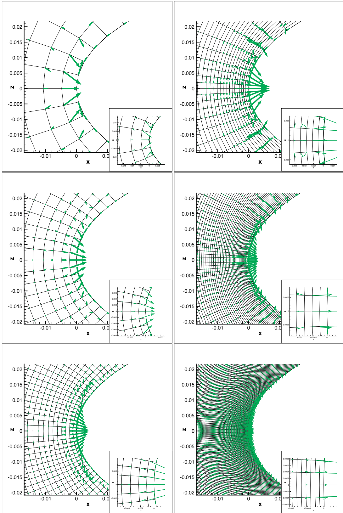
Figure 6: NACA0012, subcritical flow conditions. Examination of \mathcal{P}(dP_a/dX) for (129 \times 129) (top) (257 \times 257) (middle) (513 \times 513) down for quasi-uniform (left) and stretched mesh (right) for Roe's scheme (same scale for all plots).
