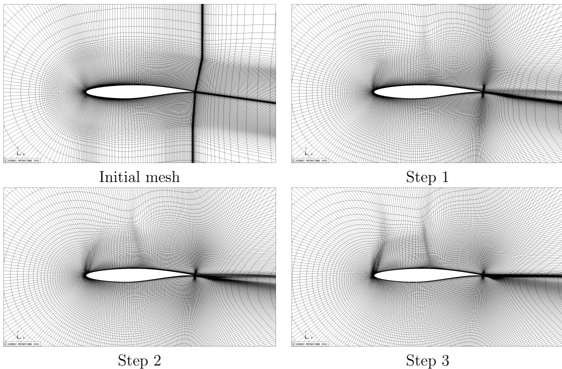
Figure B.3: Meshes during the feature-based adaptation process, M_\infty = 0.725 , \text{AoA} = 2.466^\circ , \mathcal{R}e/m = 6.5 \cdot 10^6
