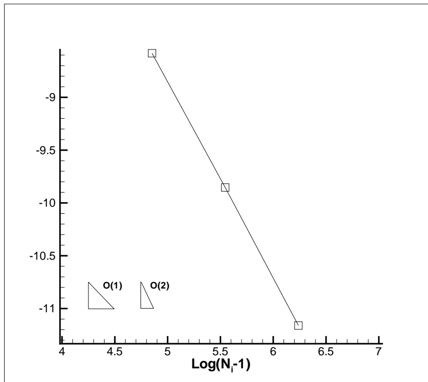
Figure 4: NACA0012. Subcritical flow. Quasi-Uniform meshes (129×129) (257×257) (513×513). \text{log} of mean of \|\Lambda_{CDp} \frac{dR}{dX}\| over the mesh
