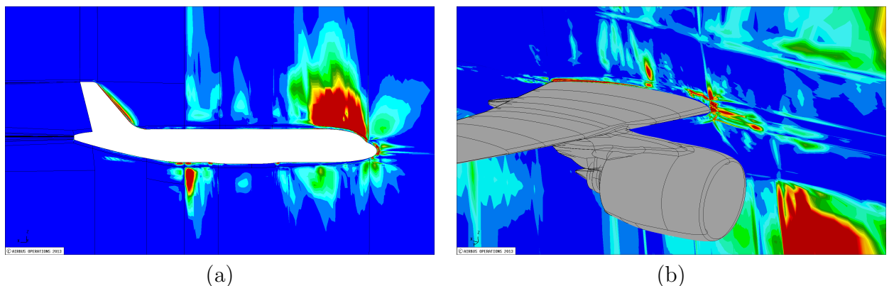
Figure 4.22: Criterion \theta for the drag ; (a) Symmetry plane ; (b) Plane between the engine and the fuselage
