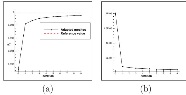
Figure 20: Results over the adaptation process for the computation of P_a for the subsonic test case. (a) P_a values (b) \bar{\theta}[P_a] values.
