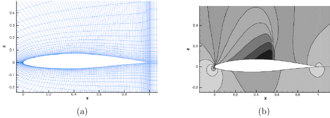
Figure 2.2: (a) C-type grid around the NACA64A212 airfoil (size 257) (b) Isochores of a Eulerian flow with M_\infty = 0.75 , AoA = 2.5^\circ
