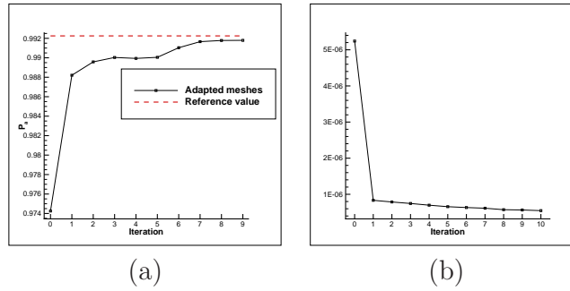
Figure 22: Results over the adaptation process for the computation of P_a for the transonic test case. (a) P_a values (b) \theta[P_a] values.
