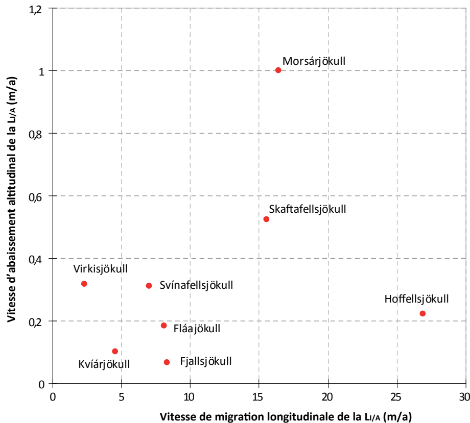
Figure R28 - Vitesses de migration aval de la L_{I/A}
