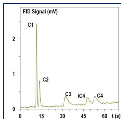
GeoService1, semi-packed column (1.1 m x 200 \mu\text{m} x 100 \mu\text{m} , e_f=1 \mu\text{m} ), P=6.8 bar, V_{inj}=2 \mu\text{L} , T=10^\circ\text{C}-120^\circ\text{C} at 6^\circ\text{C/s} .
