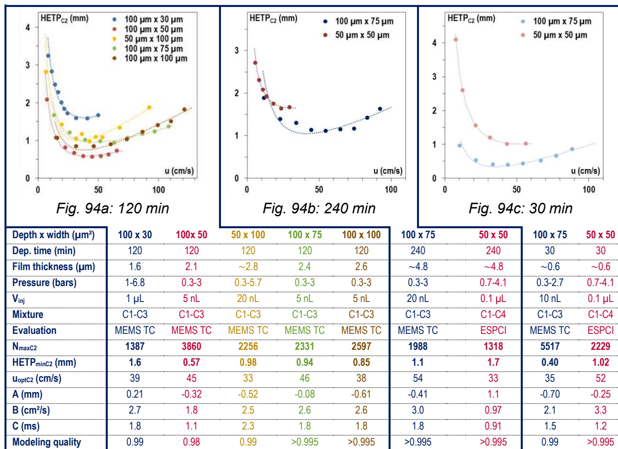
Fig. 94: influence of column section (at identical deposition times) on kinetic performances for 2.2 m-long open silica columns, T=30^\circ\text{C}
