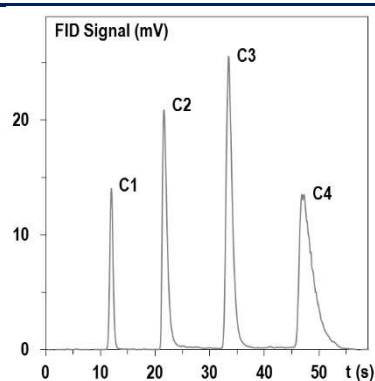
Fig. 103b: C1-C4, semi-packed column (1.1 m x 200 \mu\text{m} x 100 \mu\text{m} , e_f=0.1 \mu\text{m} ), P=6.8 bar, V_{inj}=2 \mu\text{L} , T=30^\circ\text{C}-120^\circ\text{C} at 3^\circ\text{C/s} .
