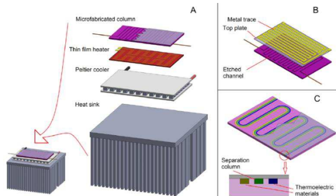
Fig. 30b: micro column temperature-programming systems, as summarized by Wang [44] (A: external heater, B: on-chip heater, C: internal heating and cooling with Peltier strips)
