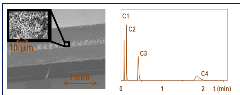
Fig. 36: micro column with monolithic porous silica, SEM image (left) and C1-C4 separation (right), by Azzouz [97]
