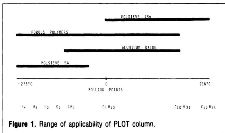
Figure 20: range of applicability of molecular sieve, porous polymer and alumina PLOT columns, according to Henrich [24]
