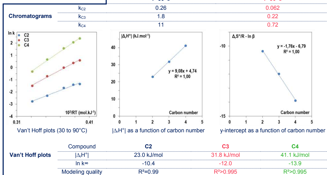
Fig. 84 : thermodynamic evaluation of a silica regular column, 2.2 m x 100 \mu\text{m} x 100 \mu\text{m} , e_r \sim 2.6 \mu\text{m} P=5.1 bars, evaluation at MEMS TC, C1-C2-C3-C4 mixture, V_{inj}=5 nL
