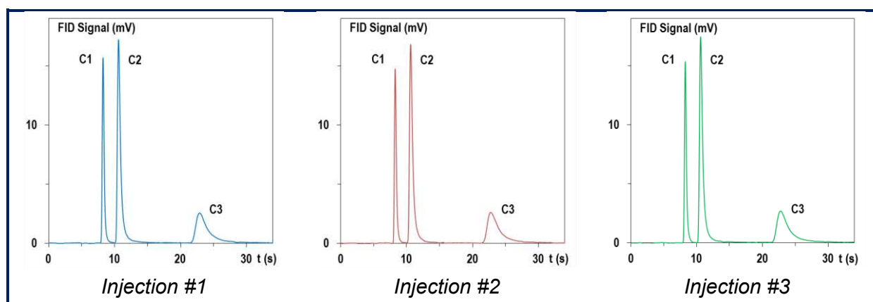
Fig. 75: C1-C2-C3 separations on a silica regular column (2.2 m x 100 \mu m x 100 \mu m, \epsilon_f=2.6 \mu m) 3 injections in a row P=0.7 bar, T=30^\circ\text{C} , V_{inj}=5 nL with Varian GC 3800
