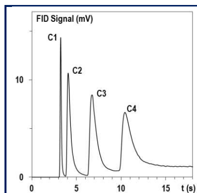
Fig. 103a: C1-C4, open regular column (2.2 m x 100 \mu\text{m} x 100 \mu\text{m} , e_f=0.8 \mu\text{m} ), P=6.8 bars, V_{inj}=20 nL, T=30^\circ\text{C}-120^\circ\text{C} at 10^\circ\text{C/s} .
