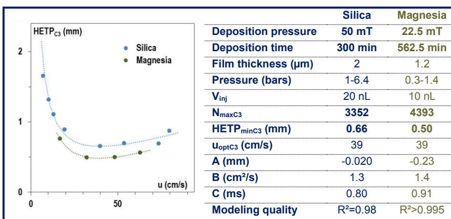
Fig. 101: influence of target material chosen for stationary phase sputtering deposition : silica and magnesia; open regular columns 2.2 m x (100 x 100) \mu\text{m}^2 , evaluation at MEMS TC, T=30^\circ\text{C} .
