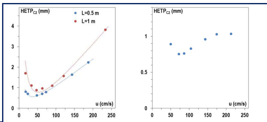
Fig. 93a: compared evaluation (MEMS TC)
