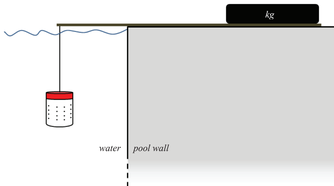
Figure 5: Experimental setup for the experiment "magnetoreception": the perforated plastic barrel hanging 40 cm from the pool wall at a depth of 50 cm, attached to a wooden plank (covered with neoprene to avoid injury and weighted down with a 10 kg block).
