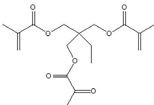
Trimethylolpropane trimethacrylate (TRIM)
