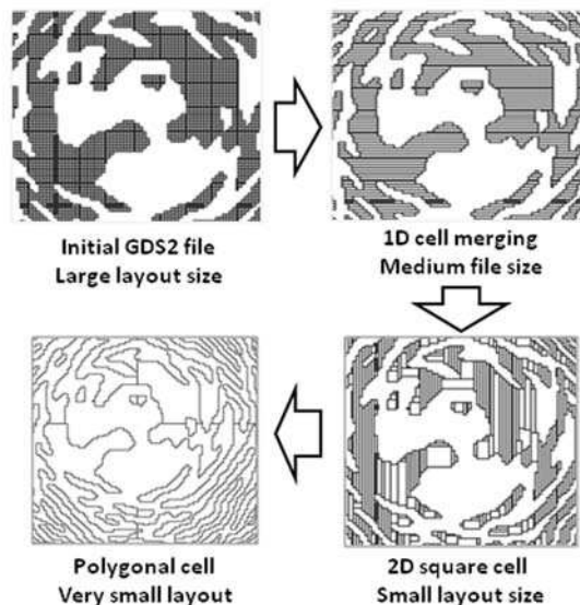
Fig. 2. Vector fracture of binary black and white file into optimized GDS2 file.
