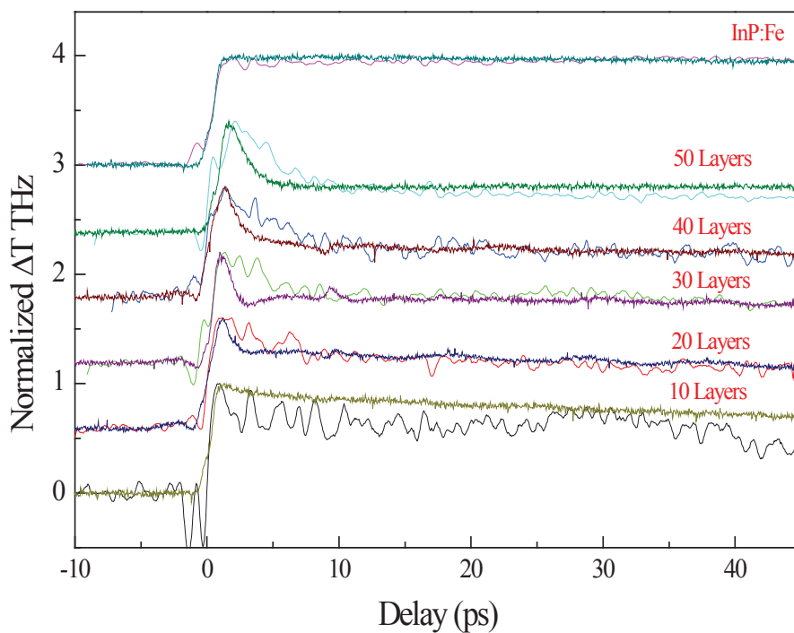
Fig. 5.27b: Corrected variation of THz transmission done for another setup at 0.8 \mu\text{m} .
