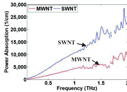
Figure 6. Power absorption of the SWNTs and MWNTs thin films.
