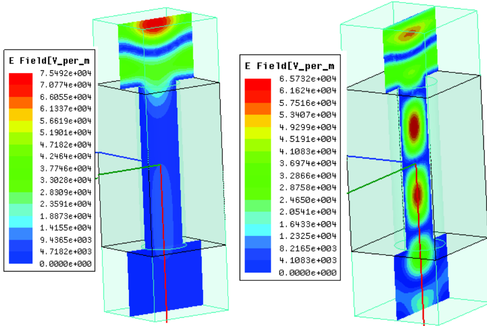
Fig. 5.12b: HFSS electrified mapping at 3.34 THz (left: below cutoff frequency f_c=3.45 THz) and at 0.4 THz (right: above cutoff) in unit cell.
