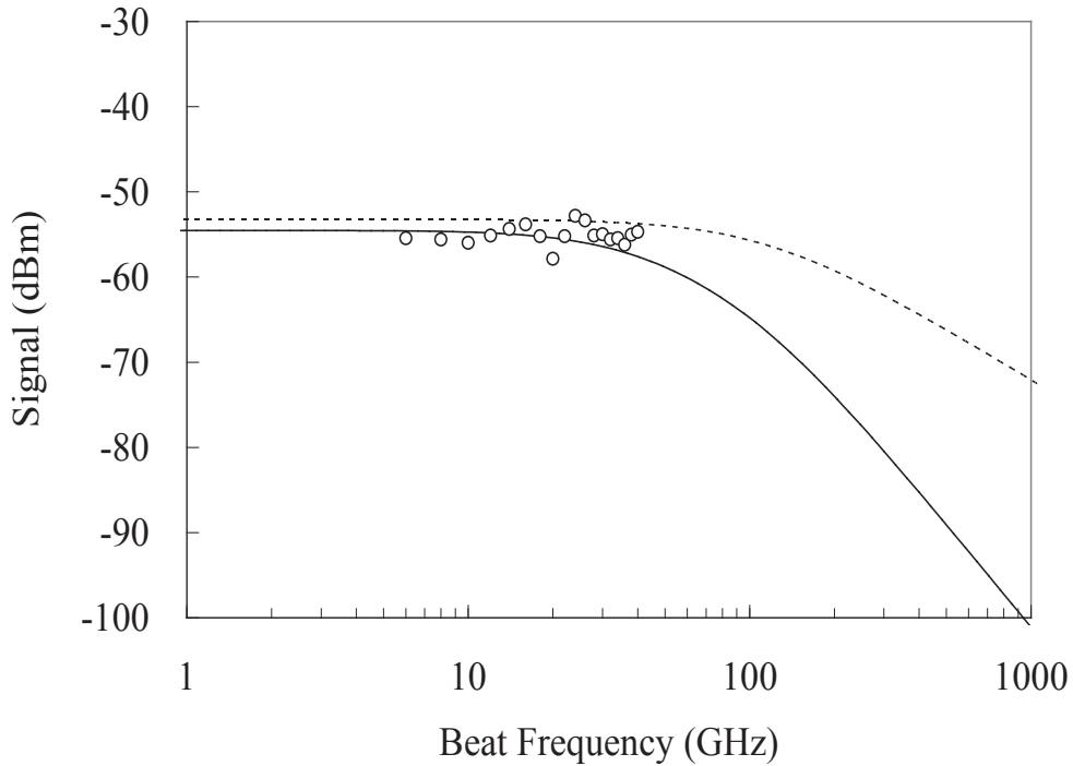
Fig. 2.16: Powers at \omega - \Omega delivered by the device versus the optical beat frequency f_{\Omega} . f_{\omega} = 20 GHz, P_{RF} = -10 dBm, P_o = 22 mW. The line is calculated with (II-31). Open circles are measured data. The dashed line is the power P_{\Omega} generated when a DC voltage ( V_{DC} = 1 V) is applied to the device.
