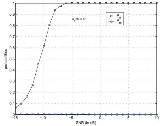
(b) Detection and false alarm probabilities P_d and P_{fa} versus SNR, for e_\sigma = 0.0001
