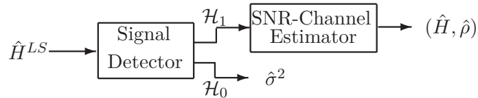
FIGURE 4.26 – Diagram of the proposed algorithm, usable as detector and estimator.
