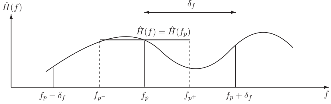
FIGURE 2.8 – Illustration of nearest-neighbor interpolation.
