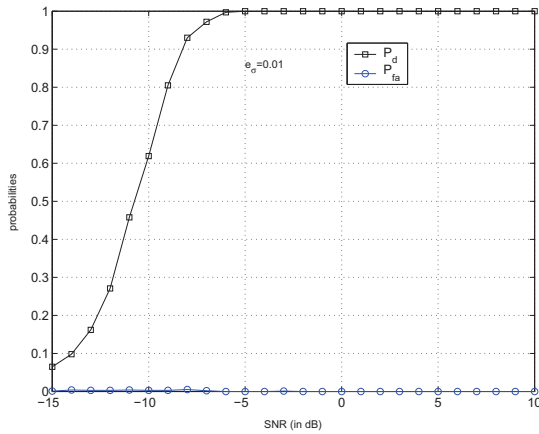
(a) Detection and false alarm probabilities P_d and P_{fa} versus SNR, for e_\sigma = 0.01
