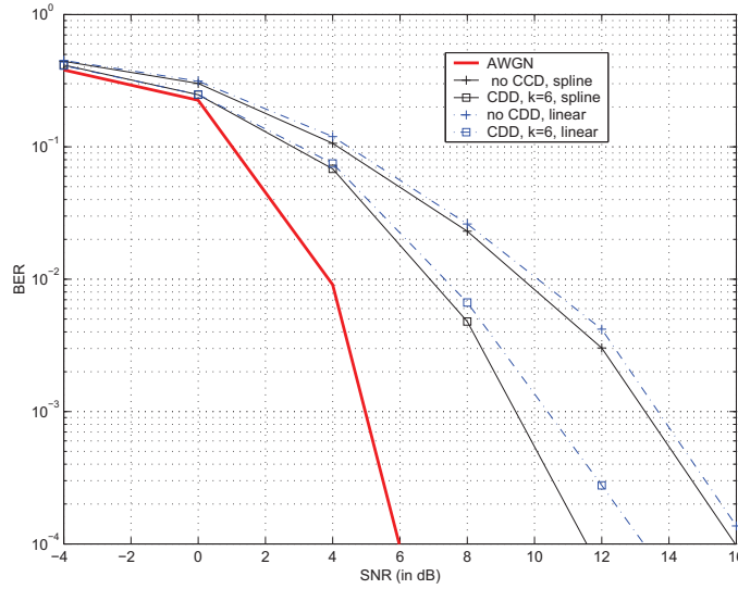
FIGURE 6.16 – BER versus SNR, effect of the interpolation, with and without CDD.
