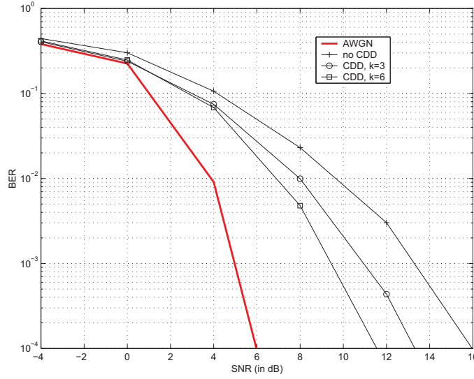
FIGURE 6.15 – BER versus SNR for transmissions with and without CDD.
