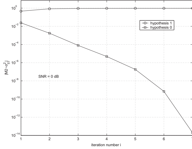
FIGURE 4.21 – |M_2 - \hat{\sigma}^2| versus the iterations number under \mathbb{H}_0 and \mathbb{H}_1 , for \text{SNR} = 0 dB.
