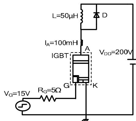
Figure 3.4 Circuit de simulation
