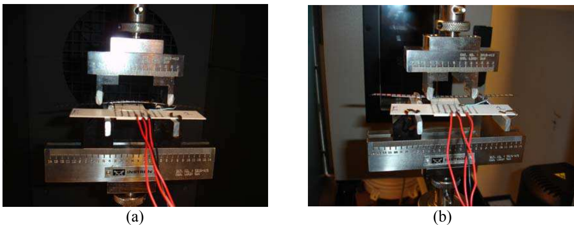
Figure 5.20 Lamelles de transistors sous flexion (a) Traction - compression, (b) Compression – traction
