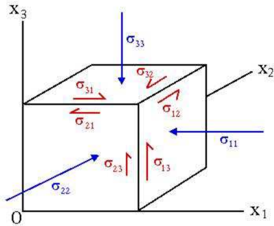
Figure 2.1 Directions des contraintes
