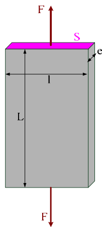
Figure 4.6 Traction uniaxiale
