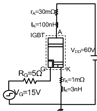
Figure 3.10 Circuit de simulation
