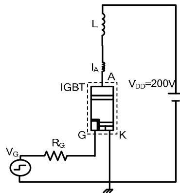
Figure 3.7 Circuit de simulation
