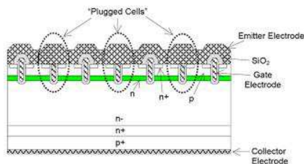
Figure 1.17 Technique PCM de MITSUBISHI ELECTRIC [Mits]
