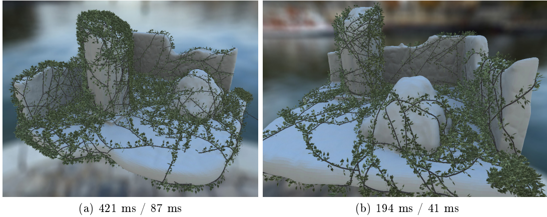
Figure 6.15: The ruins model is covered by 18 (a) and 24 (b) ivy plants, with grammar parameters stepNumber = 34/48(a/b) , stepSize = 10/13 , stepBranch = 6/14 and numberOfLeaves = 2/2 . Respectively 5.17M and 2.27M polygons are generated. Timings are indicated as rule expander / terminal evaluation and rendering.
