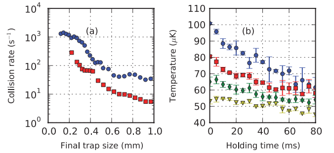
FIG. 15. (Color online) (a) Elastic s -wave collision rate as a function of the trap size after compression. The blue points correspond to a 5 ms compression and 2 \times 10^7 atoms initially loaded. The red squares correspond to a 10 ms compression and 10^7 atoms initially loaded. (b) Temperature as a function of the holding time for different initial conditions of the atoms in the dipole trap. The different initial conditions are prepared by compressing the cloud during 40 ms from an initial size L_i = 1 \text{ mm} to different final trap sizes after compression, L_f = 0.42 \text{ mm} (blue points), 0.47 \text{ mm} (red squares), 0.52 \text{ mm} (green diamonds), and 0.57 \text{ mm} (yellow triangles). After compression the diameter is kept constant. The state of the system after compression is used as the initial condition for this measurement. The smaller is the trap size after compression, the hotter and denser are the cloud initial conditions. The initial densities and temperatures are 1.7 \times 10^{11} , 1.6 \times 10^{11} , 1.4 \times 10^{11} , 1.2 \times 10^{11} \text{ cm}^{-3} and 101, 81, 65, 53 \mu\text{K} , which correspond to elastic s -wave collision rates of 27, 23, 17, 14 \text{s}^{-1} , respectively. These s -wave collision rates are compatible with the points showing the temperature reduction. Parameters: P = 200 \text{ mW} , \Delta = 40 \text{ GHz} , w = 65 \mu\text{m} , and f_m = 90 \text{ kHz} .
