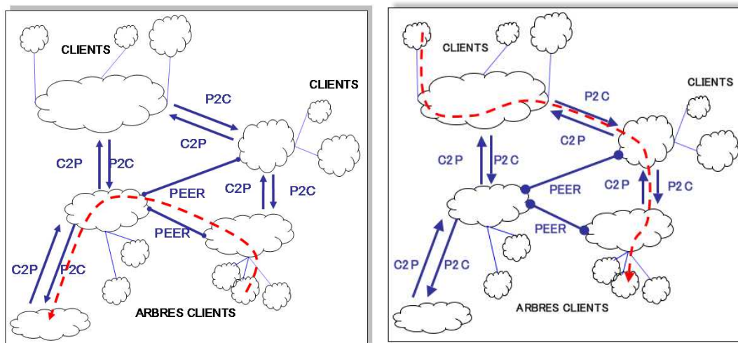
(a) Cheminement valide (1)
