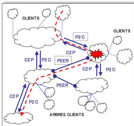
(e) Cheminement invalide (2)
