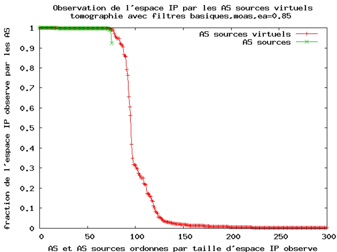
(a) tomographie T_{2005-01}
