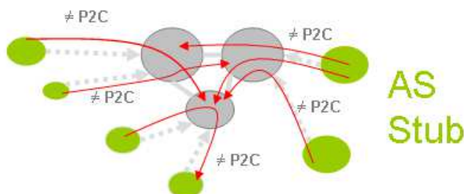
FIG. 3.6 – Illustration des contraintes C_{stub}
