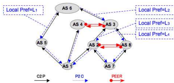
(a) graphe des AS
