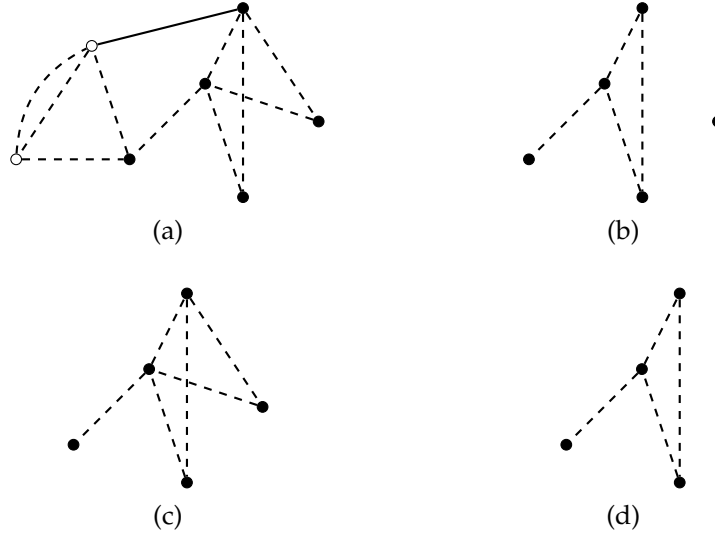
Figure 2: (a) A graph G = (V, E) where the black vertices define a set U \subseteq V and the dashed edges define a set F \subseteq E . (b) The subgraph (U, F) of G . (c) The subgraph G[U] induced by U . (d) The subgraph G[F] induced by F .
