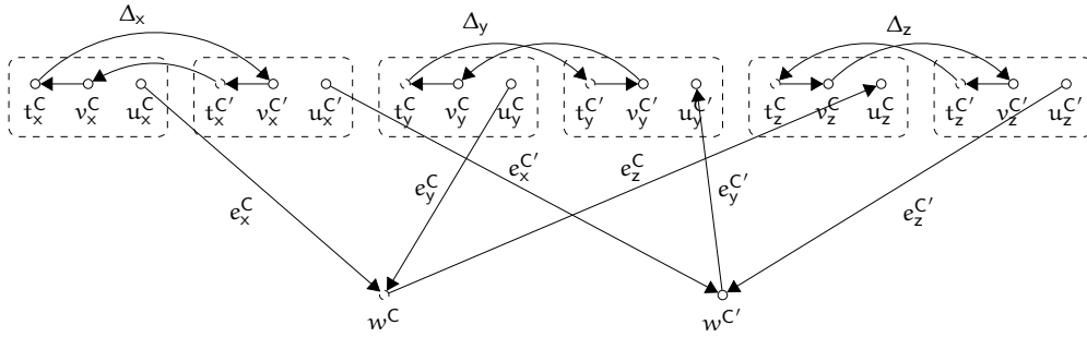
Figure 20: Representation of the circuits and the special arcs of D_3(\Pi) where \Pi is composed of the clauses C = (x, y, \bar{z}) and C' = (x, \bar{y}, z) . The dashed boxes represent the clause-variable gadgets.
