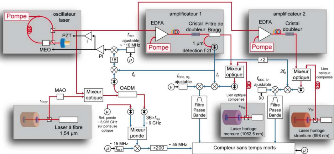
Figure 1.3: Schematics of the setup of the Er-doped fiber based optical frequency comb currently used at LNE-SYRTE for optical frequency measurements.
