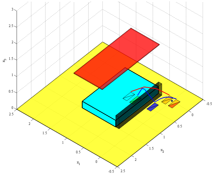
Figure 6.7: The end-effector trajectories (for left foot and right foot) are shown in this figure. The reference point are chosen to be the ankles of the feet that are 10cm higher over the sole. The blue trajectory for the left foot consists of two steps: the first one is generated by parametric curve and the second one is generated using Bi-RRT approach. The red trajectory for right foot consists of only one step and it is generated by Bi-RRT approach.
