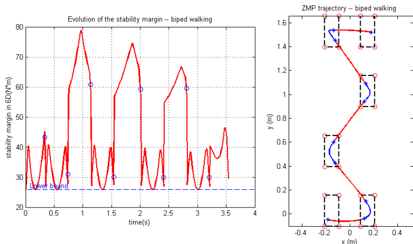
Figure 5.13: Left: stability margins of the generated biped walking motion. Right: Footsteps and the trajectory of ZMP computed from the result CoM trajectory (double-support phases in red, single-support phases in blue). Instants of support change are indicated by * in this figure.
