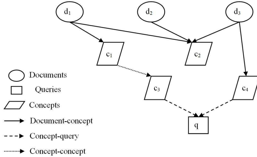
Figure 2.3: Bayesian Network of Diem Le
