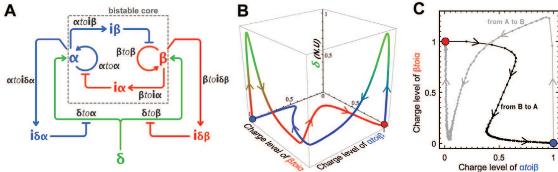
Figure 3.7: (A) Circuit of the push-push memory: a single external input \delta controls the bistable core. (B) Calculated 3D trajectories in the space \{\text{Charge level of } \alpha to i\delta\alpha, \text{ Charge level of } \beta to i\delta\beta, \text{ Normalized total concentration of } \delta\} for the push-push memory switching from A to B (blue) and B to A (red). Normalized values of \delta (injected as a gaussian spike) from 0 to 1 are associated to a color gradient from blue/red to green. (C) Experimental trajectories of the push-push memory circuit showing two independent experiments: one where the system is initially set on the state A, then flipped to B upon injection of 30 nM of \delta , and another where the same system is set in state B, then flipped to A upon injection of the same input. The charge level of \beta to i\delta\beta higher than 1 indicates that the amount of \beta transiently produced by activation module \delta to \beta during switching exceeds the concentration of \beta at the stable state B.
