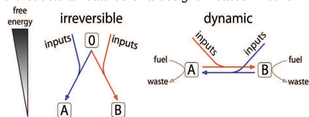
Figure 1: Irreversible system versus dynamic system. (Left) From an initial state (0) and a set of inputs, an irreversible system evolves towards a low-potential equilibrium state that corresponds to the answer of the computation (A or B), and cannot be re-used. (Right) A dynamic system continuously consumes energy. Upon reading of a set of inputs (that may be endogenous), it transits from state to state, but does not get trapped in the equilibrium: it can be re-used or perform recursive tasks.
