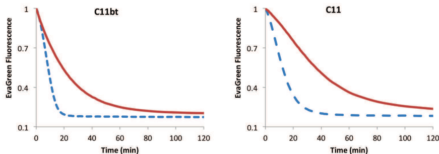
Figure 4.3: Comparison of RecJ f and cd-ttRecJ. Degradation of two non-protected substrates with RecJ f (dashed, blue curves) and cd-ttRecJ (red, solid curves). Whereas RecJ f shows a typical Michaelis-Menten kinetic, cd-ttRecJ seems to have a first order kinetic in these conditions. This reaction was performed at 38 °C with 500 nM of substrate, with a concentration of cd-ttRecJ of about 50 nM.
