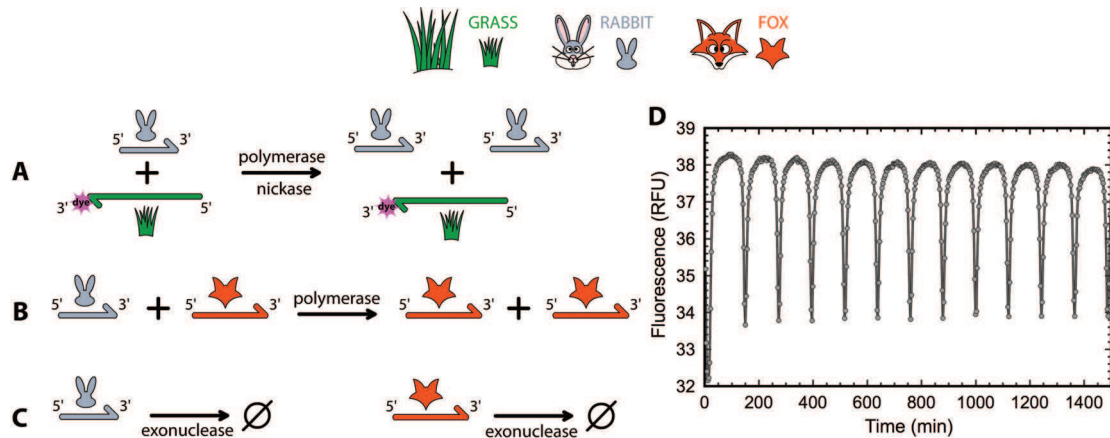
Figure 6.1: DNA-based Predator-Prey system. (A) In presence of the grass DNA template, rabbits autocatalytically reproduce. (B) Predation of rabbits by foxes. (C) Death of both rabbits and foxes. (D) Experimental curve in 0-dimensional milieu (test tube) using N-quenching [147], showing oscillations of rabbit population: a decrease in fluorescence intensity indicates an increase in rabbit concentration.
