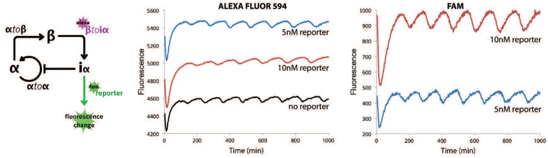
Figure 2.14: Monitoring C11bt oligator with the reporter of inhibitor. (Left) Circuit of the oligator. \beta to i \alpha is labeled with Alexa Fluor 594, thus reporting the presence of \beta . i \alpha can hybridize to the reporter, which is labeled with FAM. (Middle) Looking at the Alexa channel: the presence of increasing concentration of reporter seems to slow down the oligator (period = 113 min with reporter, 122 with 5 nM and 148 with 10 nM of reporter). (Right) Looking at the FAM channel: the reporter successfully reports on the presence of inhibitor i \alpha . The experiment was run without EvaGreen, at 37.5 °C, and with \alpha to \alpha = 30 nM, \alpha to \beta = 3 nM and \beta to i \alpha = 30 nM. Duplex i \alpha :reporter has a predicted T_m of 39.3 °C, to be compared with 46.7 °C for \alpha to \alpha - i \alpha . The sequence of reporter is as follows: 5'-C*T*C*AGCTTAGAC-3'-FAM.
