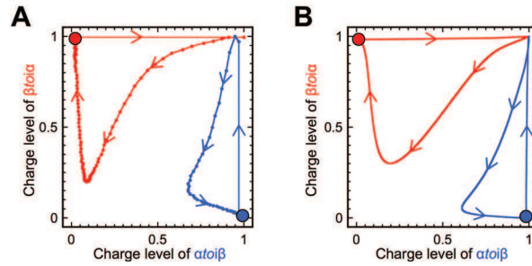
Figure 3.4: Perturbation of the bistable at the steady state. The red dot (charge level \{\alpha to \beta, \beta to \alpha\} = \{0, 1\} ) corresponds to stable state B. The blue dot (charge level \{\alpha to \beta, \beta to \alpha\} = \{1, 0\} ) corresponds to stable state A. (A) Experimental and (B) calculated (using the detailed model) trajectories of the bistable perturbed by 100 nM of the opposite input.
