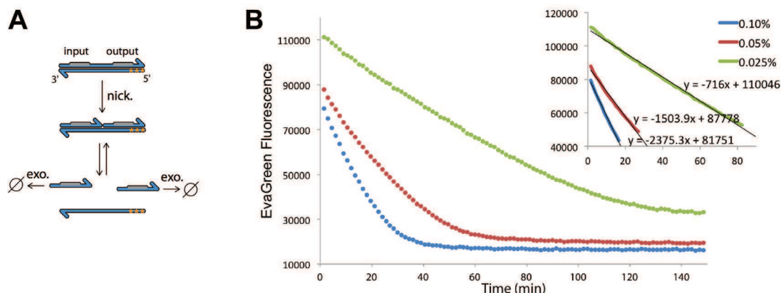
Figure 4.20: Measuring Nt.BstNBI parameters for cT11. (A) Schematic of the reaction: the template and its complementary strand are initially hybridized. The nickase cuts the complementary strand in its middle, and since the two products are shorter, they melt and are then digested by ttRecJ, resulting in a decrease of fluorescence of EvaGreen. The presence of a U in the output site of the template prevents the nickase to stick to it, which would hinder the melting of the output strand. (B) Experiment for cT11 (100 nM) with its complementary (110 nM) at 42 °C. Exonuclease is in excess (4 % of ttRecJ/160), and Nt.BstNBI is present in low concentration (0.1 % (blue), 0.05 % (red) and 0.025 % (green)). The linear portion of the curves is also displayed in inset, with the corresponding linear fit: slope of (0.05 %) is twice that of (0.025 %). However, the slope of (0.1 %) is lower than twice that if (0.05 %), meaning that the cutting reaction is not the speed limiting one anymore: this curve cannot be used to extract the kinetic parameters of Nt.BstNBI.
