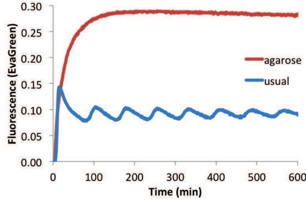
Figure D.1: Oligator c11bt with (red curve) or without (blue curve) agarose 1%. The reaction was performed at 38.4 °C. In presence of agarose, the initial amplification only performs properly. It seems that the exonuclease activity is lost.
