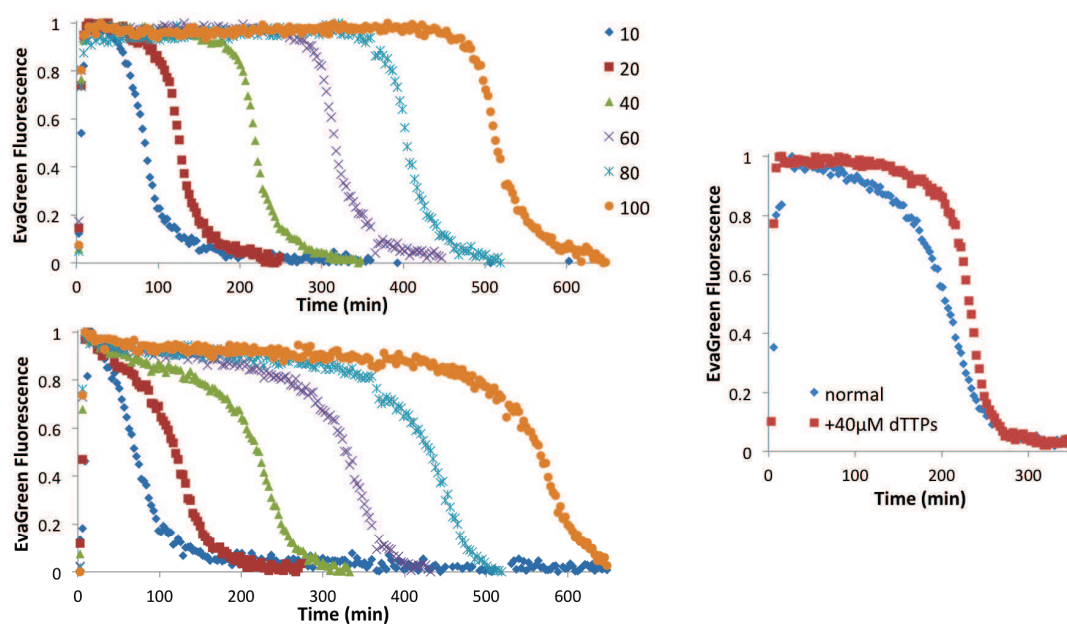
Figure 4.23: Improving the flatness of the steady state. (Left) Turnover of cX11 (up) and cV11 (down) with a ramp of initial concentration of dNTPs (from 10 to 100 \mu M). Whereas cX11 reaches a nicely flat steady state, cV11 does not, especially for the low concentrations of dNTPs. (Right) Turnover of cV11 for 40 \mu M of dNTPs. Adding dTTPs to the reaction mix improves the flatness of the steady state. Experiments were run at 43 ^{\circ} C with 20 nM of autocatalytic module.
