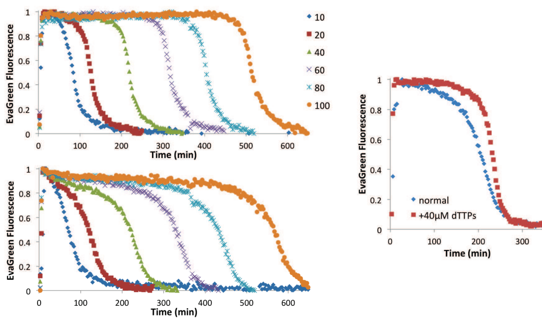
Figure 4.23: Improving the flatness of the steady state. (Left) Turnover of cX11 (up) and cV11 (down) with a ramp of initial concentration of dNTPs (from 10 to 100 μM). Whereas cX11 reaches a nicely flat steady state, cV11 does not, especially for the low concentrations of dNTPs. (Right) Turnover of cV11 for 40 μM of dNTPs. Adding dTTPs to the reaction mix improves the flatness of the steady state. Experiments were run at 43 °C with 20 nM of autocatalytic module.
