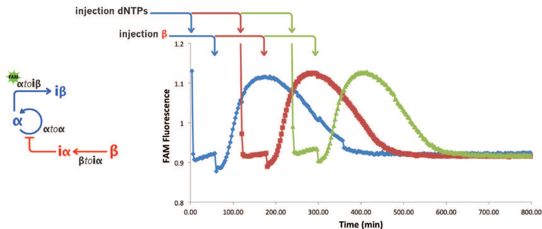
Figure 4.22: Inhibition of \alpha to \alpha (cV11, 10 nM) by \beta to \alpha (20 nM) after aging \alpha to \alpha for 0 (blue), 2 (red) or 4 hours (green). As dNTPs are injected, \alpha to \alpha starts amplifying (decrease of FAM fluorescence) reaches the steady state. After one hour, an injection of \beta (30 nM) activates the production of i\alpha , that inhibits \alpha to \alpha . This experiment was run at 43 °C.
