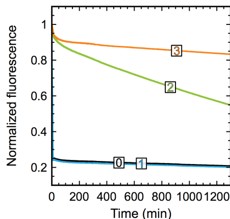
Figure 3.10: Degradation of template \beta to \beta (400 nM) by ttRecJ in the same buffer, ttRecJ concentration (50 nM) and temperature (42 °C) as for the bistable switch, memory and push-push memory experiments. Template \beta to \beta has 0, 1, 2 or 3 consecutive phosphorothioate backbone modifications at its 5' end.
