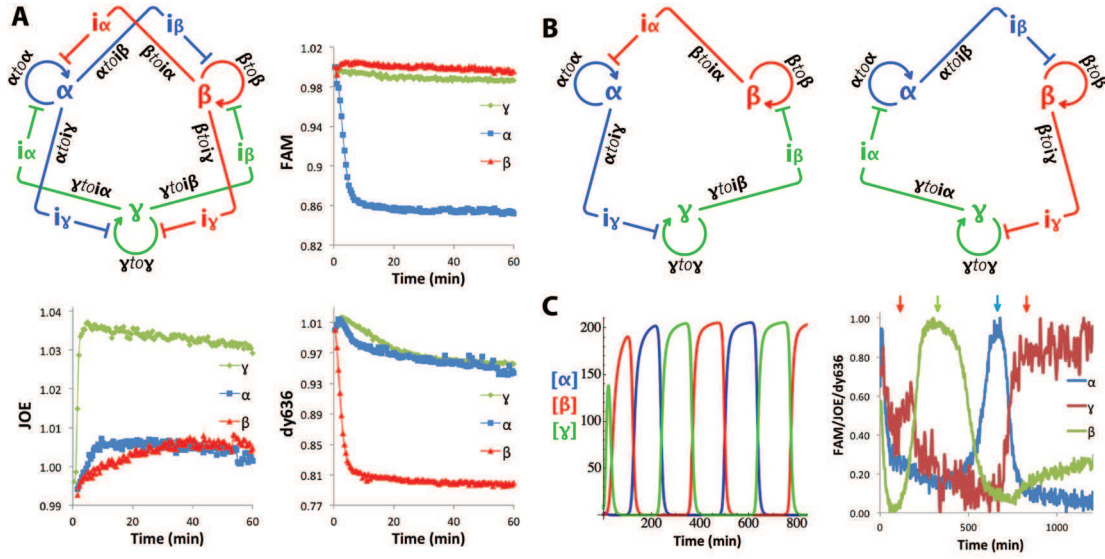
Figure 4.24: Tristability and three-switch oscillator. (A) Tristable circuit. Templates \alpha to \beta and \alpha to \gamma are labeled with FAM to monitor \alpha (negative fluorescence intensity shift upon charge); \beta to \alpha and \beta to \gamma are labeled with dy636 to monitor \beta (negative fluorescence intensity shift upon charge); \gamma to \alpha and \gamma to \beta are labeled with JOE to monitor \gamma (positive fluorescence intensity shift). The system initiated with 1 nM of either \alpha , \beta or \gamma stabilizes in each corresponding state A, B or C, characterized by a shift of fluorescence intensity of, respectively, FAM, dy636 or JOE, as one can observe in the fluorescence time plots of each dye. Concentrations are: [\alpha to \alpha] = [\beta to \beta] = 15 nM, [\gamma to \gamma] = 10 nM, all inhibition modules at 20 nM. (B) Three-switch oscillators oscillating counterclockwise (left) and clockwise (right). (C) Left: model (concentration of free \alpha (blue), \beta (red) or \gamma (green)) for perfectly equilibrated sequences all present in a 20 nM concentration. Right: experimental fluorescence (normalized, and reversed for FAM and JOE whose fluorescence change upon hybridization is negative) time plot for a system with [\alpha to \alpha] = 20 nM, [\beta to \beta] = 5 nM, [\gamma to \gamma] = 5 nM, [\alpha to \beta] = 10 nM, [\beta to \gamma] = 7.5 nM and [\gamma to \alpha] = 5 nM. This latter concentration explain the poor signal induced by \gamma . The reaction was initiated with [\gamma] = 5 nM and [\alpha] = [\beta] = 1 nM. Colored arrows indicate the successive spikes of input species: first comes a spike of \gamma , then \beta , then \alpha , after which \gamma reactivates and the system stalls forever. Sequences are as follows: \alpha : CTGAGTCTTGG, \beta : CAGAGTCCAAG, \gamma : AGGAGTCACAC.
