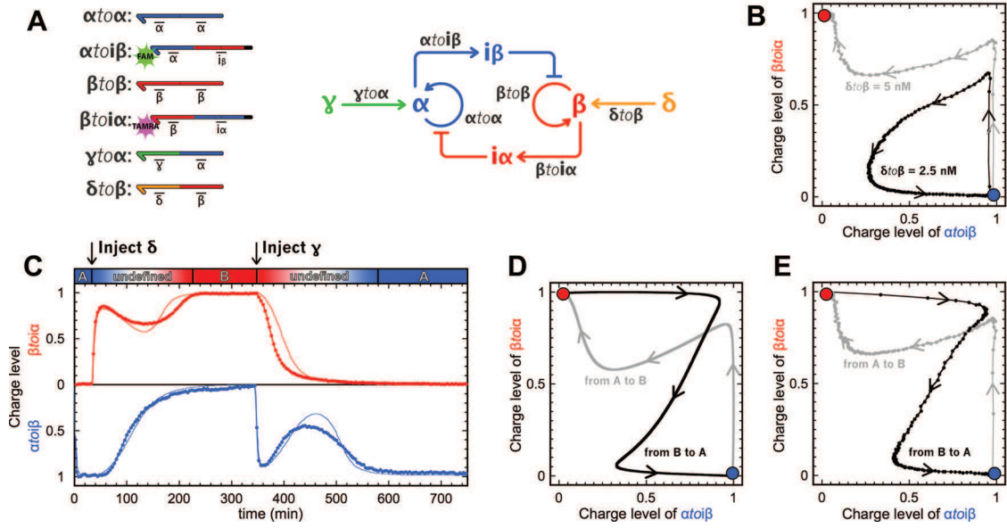
Figure 3.6: Switchable memory circuit. (A) Circuit and templates of the bistable switchable memory. (B) Trajectories of two attempts to flip the bistable memory from A to B, with \delta\alpha\beta = 2.5 nM (black, failure) and \delta\alpha\beta = 5 nM (grey, success). (C) Experimental (thick line) and fitted model (thin line) time plot of the charge levels of \alpha\text{to}\beta and \beta\text{to}\alpha . The memory circuit is started in state A, flipped from A to B, then from B to A. (D) Predicted and (E) experimental trajectories of the memory switching reversibly from A to B (grey) and B to A (black).
