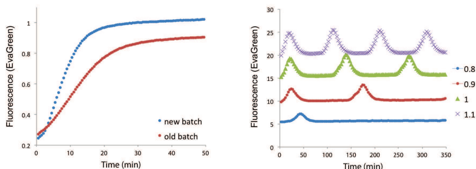
Figure 4.1: Left: Simple amplification of T11 (5'-TCGAGTCTGTT-3') in presence of 100 nM of its associated autocatalytic template. The two curves correspond to the same reaction mix to which the same concentration of Nt.BstNBI from an “old” (red) or a “new” batch was added. Fluorescence data of EvaGreen is divided by that of ROX reference dye, removing machine-related variation of fluorescence intensity. Amplification performs at a different rate, and the reactions reach a different steady state, which suggests a difference in the activity between these two batches. Right: Ramp of Bst DNA Polymerase on the oscillating system further presented in chapter 6. Curves were offset for visibility. A variation of 10 % of polymerase concentration dramatically modifies the kinetics of the system.
