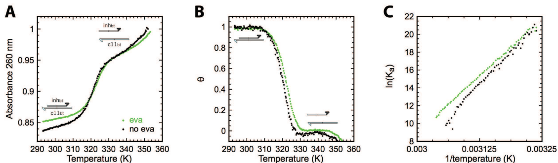
Figure 4.18: Melt curve analysis of c11bt and its inhibitor. (A) Raw melt curve with and without EvaGreen. (B) Fraction of hybridized duplex as a function of the temperature. (C) The linear fit of these two lines contains \Delta H and \Delta S of the reaction.
