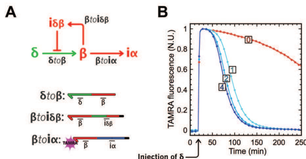
Figure 3.8: Push-push negative feedback. (A) Circuit and templates. Upon injection of \delta , production of \beta is activated. Then, \beta hybridizes to \beta to \alpha (resulting in an increase of TAMRA fluorescence) and to \beta to \beta that, in turn, produces the inhibitor of \delta to \beta , stopping the production of \beta . (B) Experimental time plot of the normalized TAMRA fluorescence (1 at the highest and 0 at the lowest) for different concentrations (0, 1, 2 and 4 nM) of inhibition module \beta to \beta .
