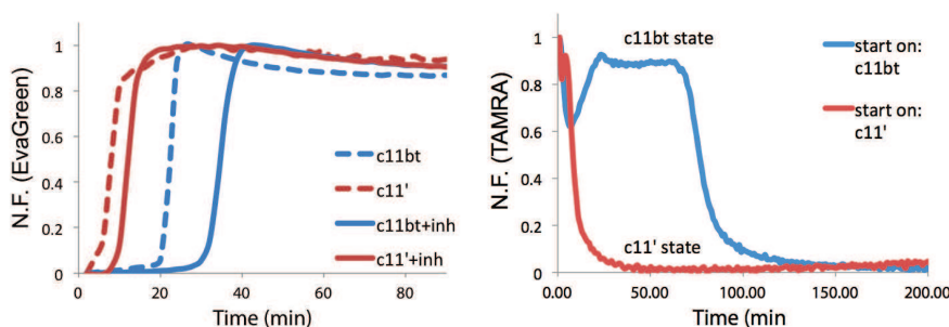
Figure 4.4: Bistable c11bt-c11' (Left) Amplification by c11bt and c11' in the absence (dashed) and presence (plain) of inhibitor strand (present in the same concentration as the autocatalytic module). In presence of inhibitor, the amplification start is delayed. (Right) Complete bistable system. Template c11' is labeled in 3' with TAMRA, which fluorescence is quenched in presence of c11' input. The system started with a small amount of input of either c11bt or c11'. Accordingly, the system takes the c11bt state (high fluorescence) or c11' (low fluorescence). However, after some time (around 70min), the system started on c11bt state self-switches toward c11' state (blue curve). These reactions were performed at 38°C, with concentration of 20nM for autocatalytic modules and 60nM for inhibitor modules.
