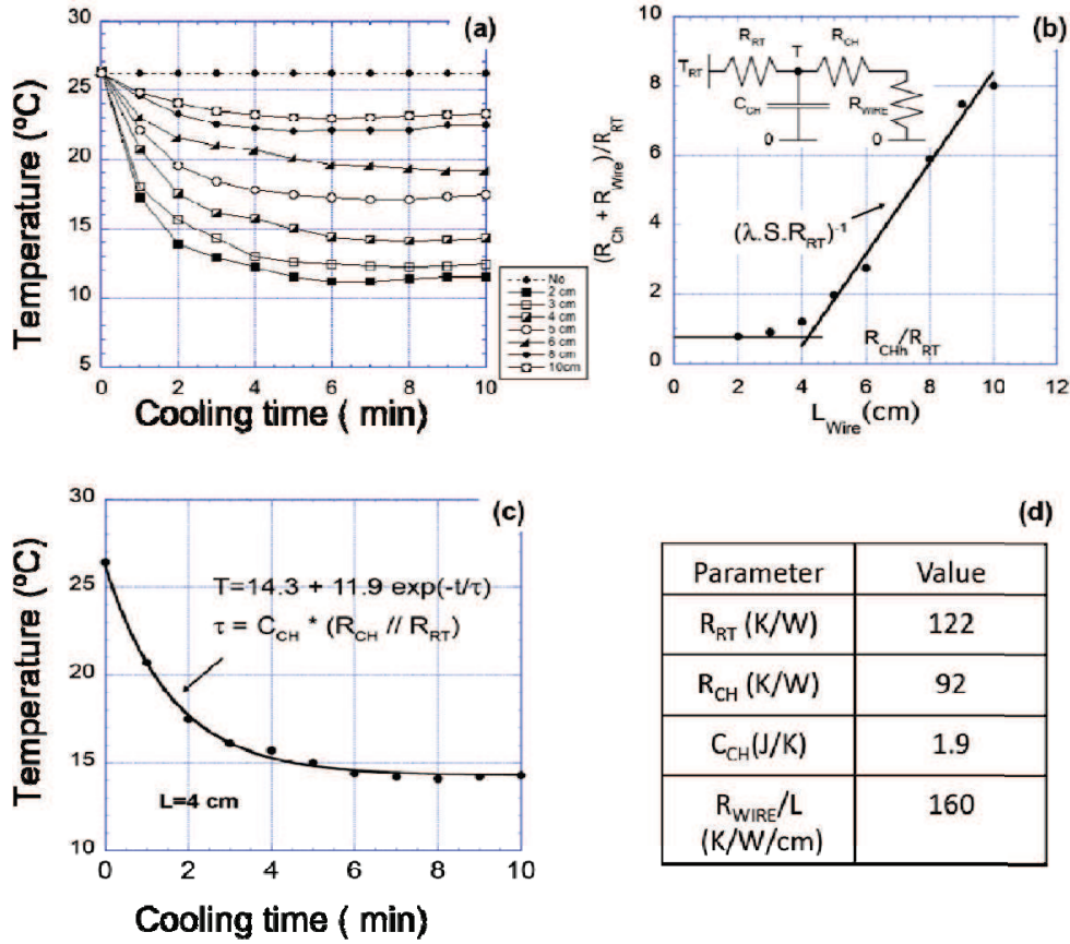
FIG. 4. Thermal characterization of the chamber. (a) Chamber temperature transients for various wire lengths. (b) Evolution of the thermal resistivity with the wire length from the steady state temperatures given by (R_{\text{CH}} + R_{\text{WIRE}}) / (R_{\text{RT}} + R_{\text{CH}} + R_{\text{WIRE}}) . (c) Transient temperature cooling with first order extraction for the determination of the response time. (d) Values of the electro-thermal equivalent parameters of the chamber and its cooling system.
