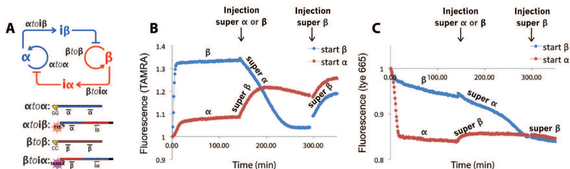
Figure 4.17: Flipping the switch with super input. (A) Bistable circuit and templates: \alpha\text{to}\alpha has two G (and \beta\text{to}\beta , two C) in 3' to receive its super input. Fluorescence of TAMRA (B) and tye 665 (C), respectively monitoring \beta (high fluorescence corresponds to high [\beta] ) and \alpha (low fluorescence corresponds to high [\alpha] ). The same reaction mix is initiated with either \alpha (red curve) or \beta (blue curve). At t = 150 min, an injection of 30 nM of either super \alpha or \beta triggers the switching process. The system initially in state B (blue curve) flips to the A state: fluorescence of TAMRA decreases (inhibition of \beta\text{to}\beta ), that of tye 665 also decreases (reactivation of \alpha\text{to}\alpha ). However, the system initially in state A (red curve) doesn't flip to state B, but seems to end up in an alternate state where both \alpha\text{to}\alpha and \beta\text{to}\beta are partially active. At t = 300 min, an injection of super \beta confirms that the system is not responsive anymore.
