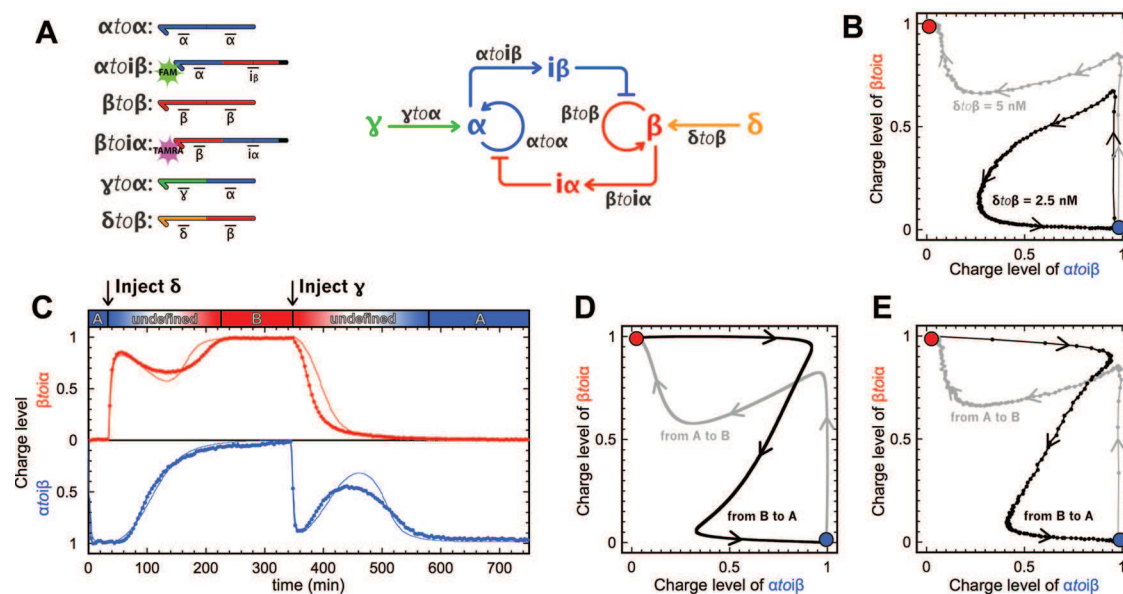
Figure 3.6: Switchable memory circuit. (A) Circuit and templates of the bistable switchable memory. (B) Trajectories of two attempts to flip the bistable memory from A to B, with \delta/\beta = 2.5 nM (black, failure) and \delta/\beta = 5 nM (grey, success). (C) Experimental (thick line) and fitted model (thin line) time plot of the charge levels of \alpha/\beta and \beta/\alpha . The memory circuit is started in state A, flipped from A to B, then from B to A. (D) Predicted and (E) experimental trajectories of the memory switching reversibly from A to B (grey) and B to A (black).
