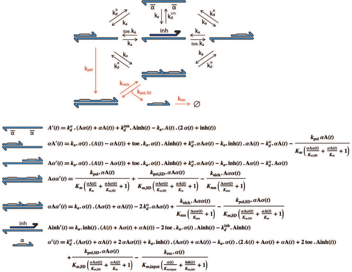
Figure 3.14: Schematic of the full set of reactions relative to a reaction circuit where input \alpha only interacts with template \alpha\text{to}\alpha , and the corresponding set of ordinary differential equations. \alpha\text{to}\alpha is noted A for simplicity of notation. Red arrows indicate enzymatic reactions. Periods indicate multiplications. Dissociation rates (in \text{min}^{-1} ) were calculated as k_d = k_a/K_d
