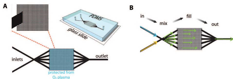
Figure 5.2: First self-closing design. (A) Device layout, 3D view and zoom on the chamber array. The latter is protected from O 2 plasma so that the liquid can make its way from the inlet to the outlet. (B) As the liquid flows from the inlet to the outlet, it fills the chambers.
