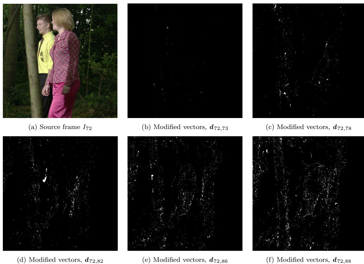
Figure 12.22: Pixels of I_{72} ( Walking-Couple-72-92 sequence) for which the from-the-reference displacement vector has been modified by the from-the-reference motion refinement described in Section 12.3.2 and involved in the two-reference frames motion refinement.
