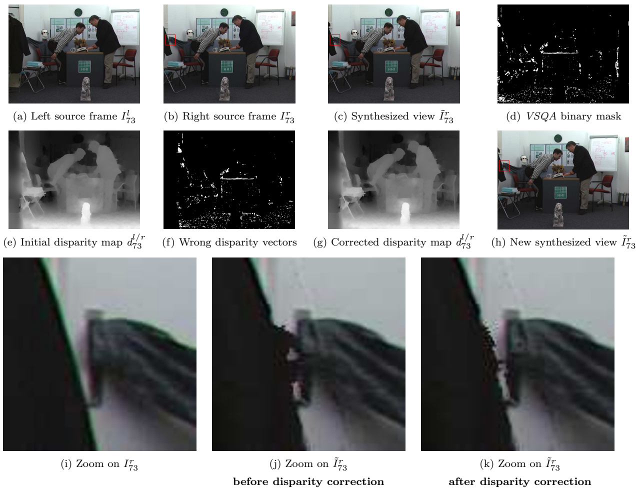
Figure 14.5: Accuracy of the proposed disparity correction framework (Section 14.2) assessed through view synthesis.
