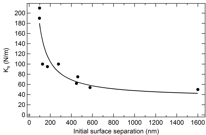
Figure 3.27: Stiffness of the sample K_s as a function of the initial separation l_0 .
