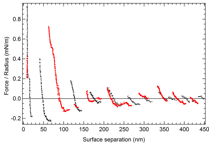
Figure 3.21: Normalized force as a function of the surface separation. The black curve is the force profile presented in Figure 3.11. The red curve exhibits exotic behavior: note the fourth oscillation with very small amplitude; the third oscillation is deformed and b = 4 .
