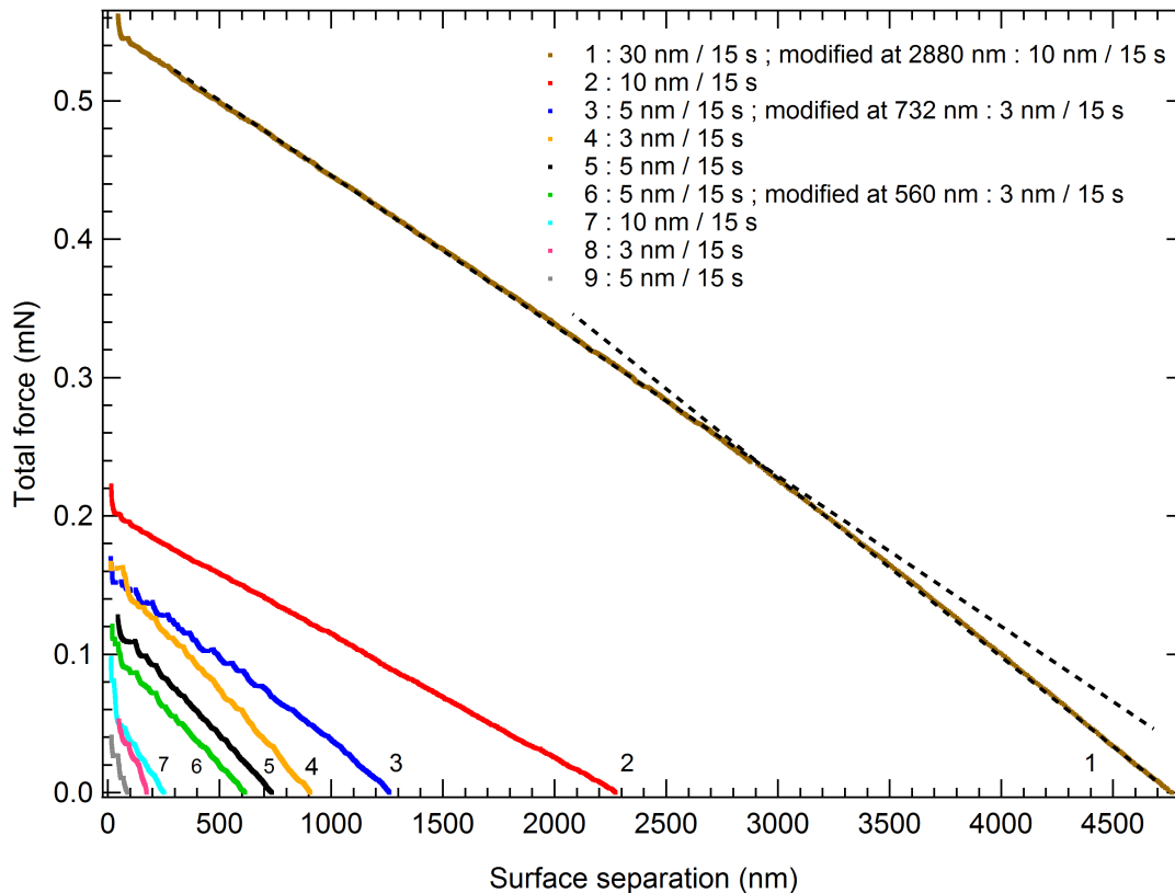
Figure 3.6: Total force as a function of surface separation for several measurements performed upon approach of the surfaces (sample L). For measurement 1, the dashed lines indicate the change in the background slope when the speed is decreased.
