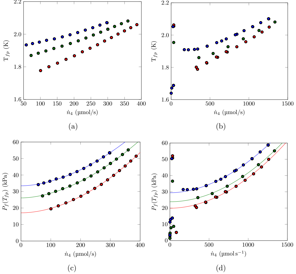
Figure 3.14: The fountain pump temperature as a function of the ^4\text{He} flow rate for two vortex capillaries of different diameter: 72\ \mu\text{m} (a) and 136.8\ \mu\text{m} (b). Panel (c) and (d) show the fountain pressure at T_{fp} as a function of the ^4\text{He} flow rate for the same vortex capillary diameters (c- 72\ \mu\text{m} , d- 136.8\ \mu\text{m} ). The different colors represent different still pressure (red points - 0.3 mbar, green points - 5.0 mbar, blue points - 10 mbar). Data for the 72\ \mu\text{m} capillary are at an overall 6 concentration of 0.1. Data for the 136.8\ \mu\text{m} capillary are at an overall concentration of 0.13 (for P_{sill}=0.3 mbar) and 0.07 (for P_{sill}=5 mbar and P_{sill}=10 mbar). In the 136.8\ \mu\text{m} curve note at low flow rates the evident change between the second and the third regimes mentioned above.
