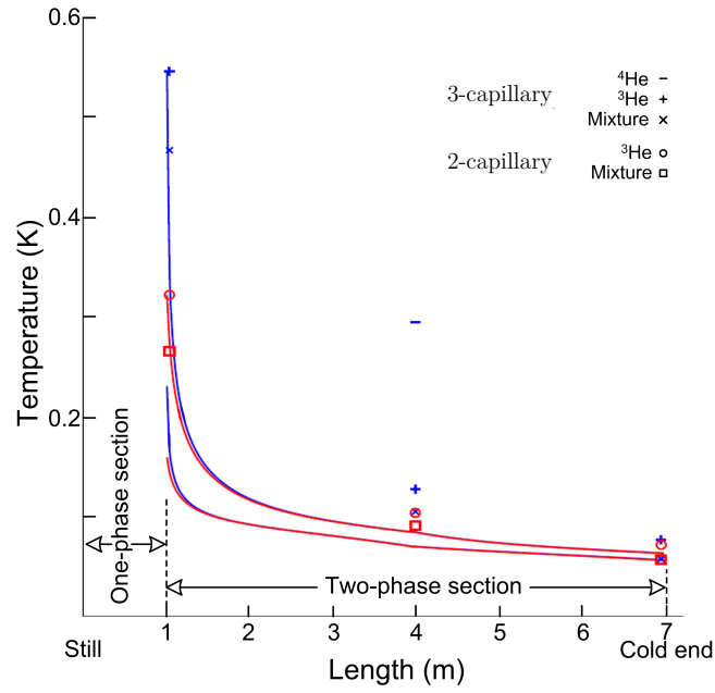
Figure 3.5: Temperature profiles for the two designs (markers) at \dot{n}_3 = 25 \mu\text{mol/s} , \dot{n}_4 = 325 \mu\text{mol/s} , T_{\text{still}} = 1.05 \text{ K} and a heat load of 1 \mu\text{W} . Also shown are the modelled profiles (blue lines - 3-capillary, red lines - 2-capillary) for the two cases. For each design the highest calculated profile is for the ^3\text{He} stream.
