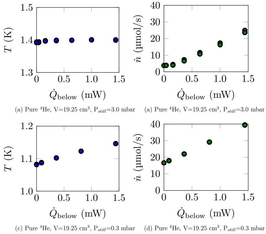
Figure B.7: Temperature T and flow rate \dot{n} as a function of the applied heating power \dot{Q}_{\text{below}} . These tests has been performed with Procelit in the fourth setup.
