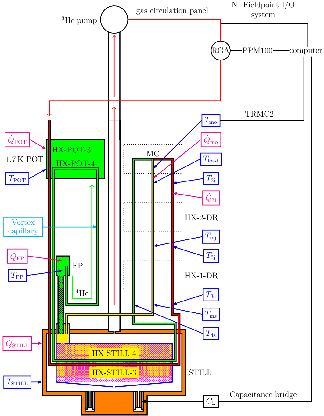
Figure 5.6: NG-CCDR test equipment. The module TRMC2 controls all the thermometers and the low temperature heaters \dot{Q}_{3i} and \dot{Q}_{mo} . The heaters \dot{Q}_{\text{POT}} , \dot{Q}_{\text{STILL}} and \dot{Q}_{\text{FP}} are controlled by the NI FieldPoint I/O system. See section 4.2.2 for the rest of the modules.
