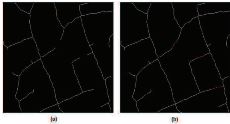
Figure 5.29 — Approximation NURBSC
