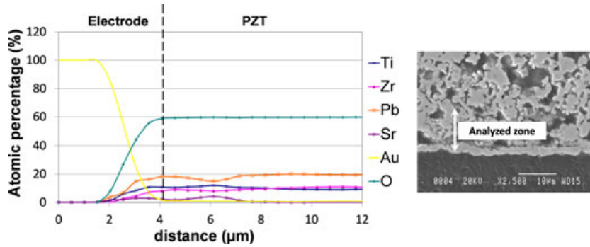
Fig. 6. X-rays microprobe analysis of the PZT/electrode interface in contact to the sacrificial layer.
