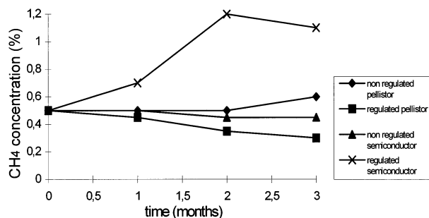
Fig. 10. Methane concentrations allowing the red LED to switch on versus time.
