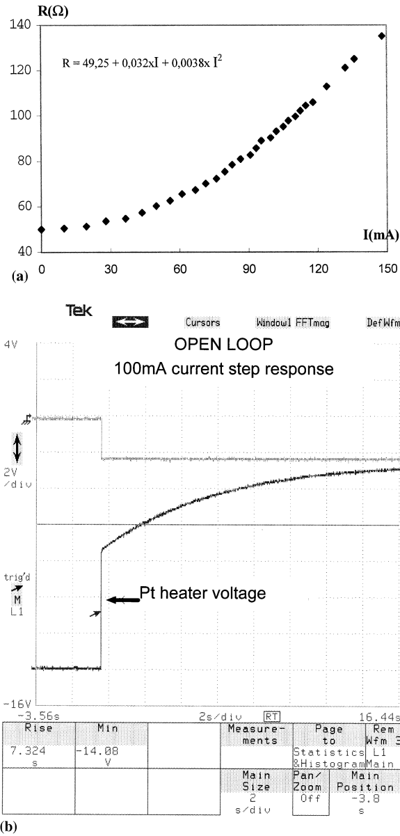
Fig. 6. Electrical characterization of the Pt resistor. (a) Static characterization; (b) dynamic characterization.
