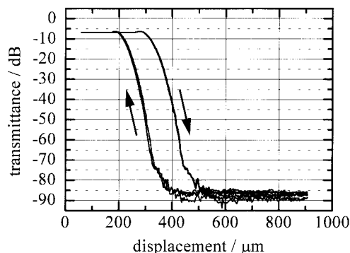
Fig. 6. Transmittance of the piezoelectric attenuator in dependence of applied external voltage; four complete cycles are shown [9].
