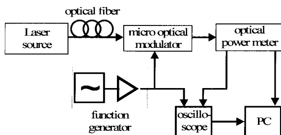
Fig. 5. Experimental setup for optical characterization of the optical attenuator [9].
