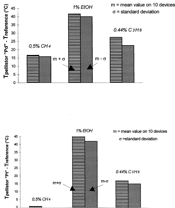
Fig. 2. Methane selectivity of the device and fabrication reproducibility (working temperature: 450°C). (a) Differential temperature T_{(pellistor \cdot Pd)} - T_{(reference)} ; (b) differential temperature T_{(pellistor \cdot Pt)} - T_{(reference)} .
