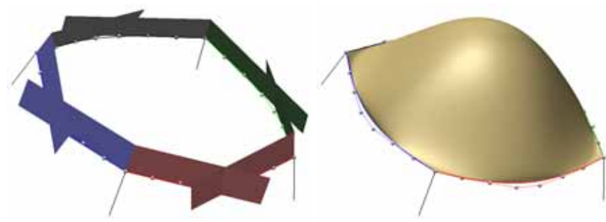
Fig. 3.24 - Left: the osculating half-planes at each corner. Right: the constructed boundary Bézier curves together with the Bézier patch interpolating these boundary curves as geodesics.
