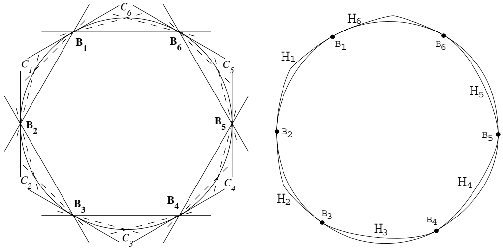
Fig. 1.15 - Interpolating oval of constant width.
