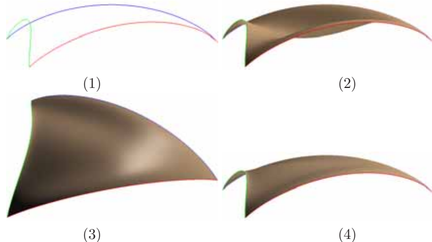
Fig. 3.21 - (1) the three boundary curves satisfying consistency conditions, and for which the corner angles sum to 2\pi ; (2) the initial reconstructed surface with free parameters equal to zero; (3) and (4) two different views of the reconstructed surface after smoothing according the thin–plate spline energy criterion.
