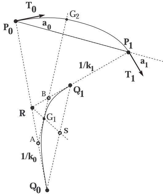
Fig. 1.4 - G^2 Hermite interpolation of admissible curvature elements by two segments of T-quartics with G^2 contact and monotonous curvature.
