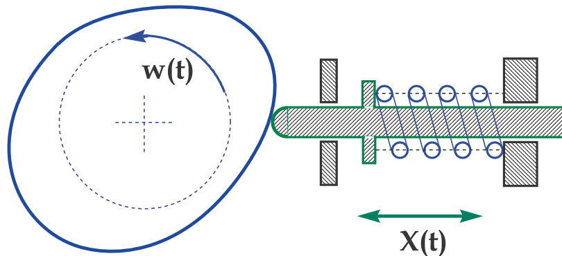
Fig. 1.7 - Cam mechanism with spring.
