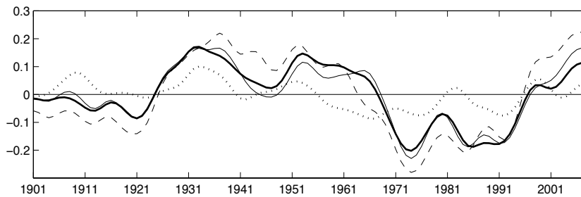
Figure 4.26: Time series in ^{\circ}\text{C} of the traditional AMO (dashed line), the AMO-GT (continuous line), the AMO-GT/EN (thick line), and the AMO-GT/EN/PD (dotted). LIM made from observed SST.
