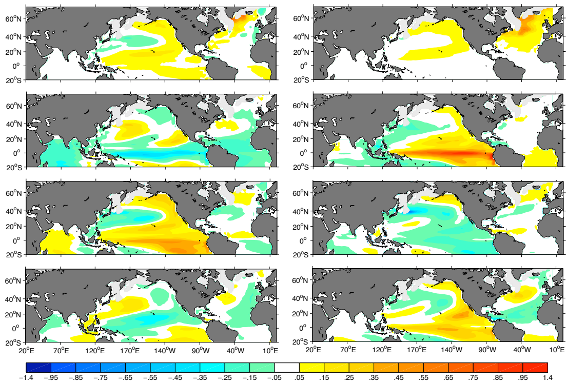
Figure 4.17: Normal modes (in °C) of the deterministic matrix B . Mode 1/2 (1st row), 5/6 (2nd row), 7/8 (3rd row), and 14/15 (bottom). LIM made from HadCM3.
