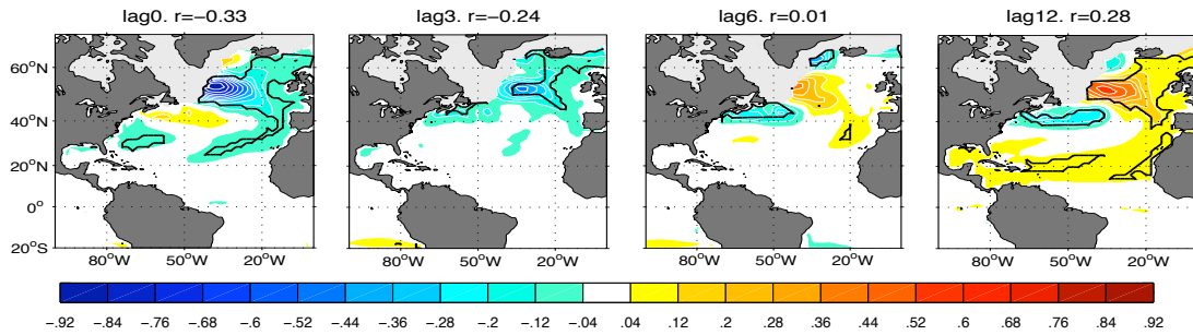
Figure 4.9: Regression of low-pass filtered SST onto AMOC PC1 in phase and when the AMOC leads (lag in yr) for the historical IPSLCM5 simulation. The black contour indicates 5% significance and r is the correlation between the 1st AMOC PC and the traditional AMO. Light gray shading indicates where the sea ice cover in March is higher than 25%.
