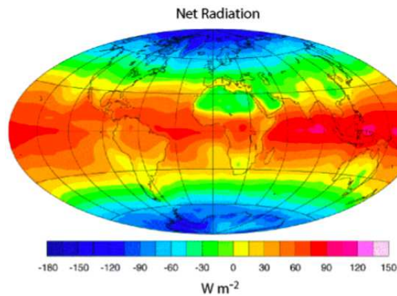
Figure 1.1: Heat flux received at the Earth surface. Source : NASA.
