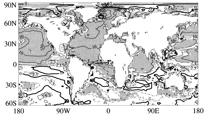
Figure 1.15: Regression of decadal averaged SST anomalies onto the AMOC maximum (units 0.01 \text{ } ^\circ\text{C}\cdot\text{Sv}^{-1} , contours values at \pm 50, 25, 10, 5, 2.5 , and 0 ). Solid contours indicate positive values and dash-dotted contours correspond to negative values. The shaded area indicates that the regression is 5% significant. Source : [Vellinga and Wu 2004].
