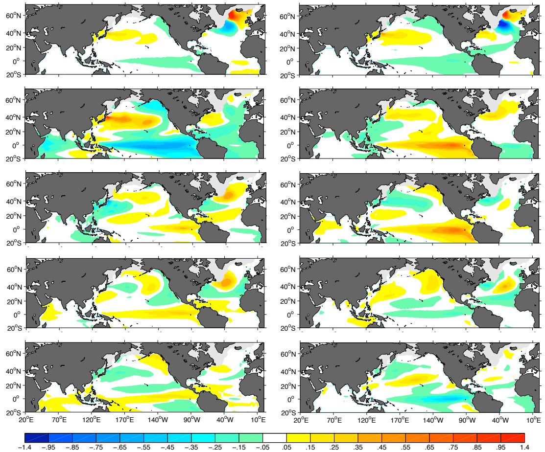
Figure 4.18: Normal modes (in ^{\circ}\text{C} ) of the deterministic matrix \mathbf{B} . Mode 1/2 (1st row), 3/4 (2nd row), 12/13 (3rd row), 17/18 (4th row), and 20/21 (bottom). LIM made from IPSLCM5 (control).
