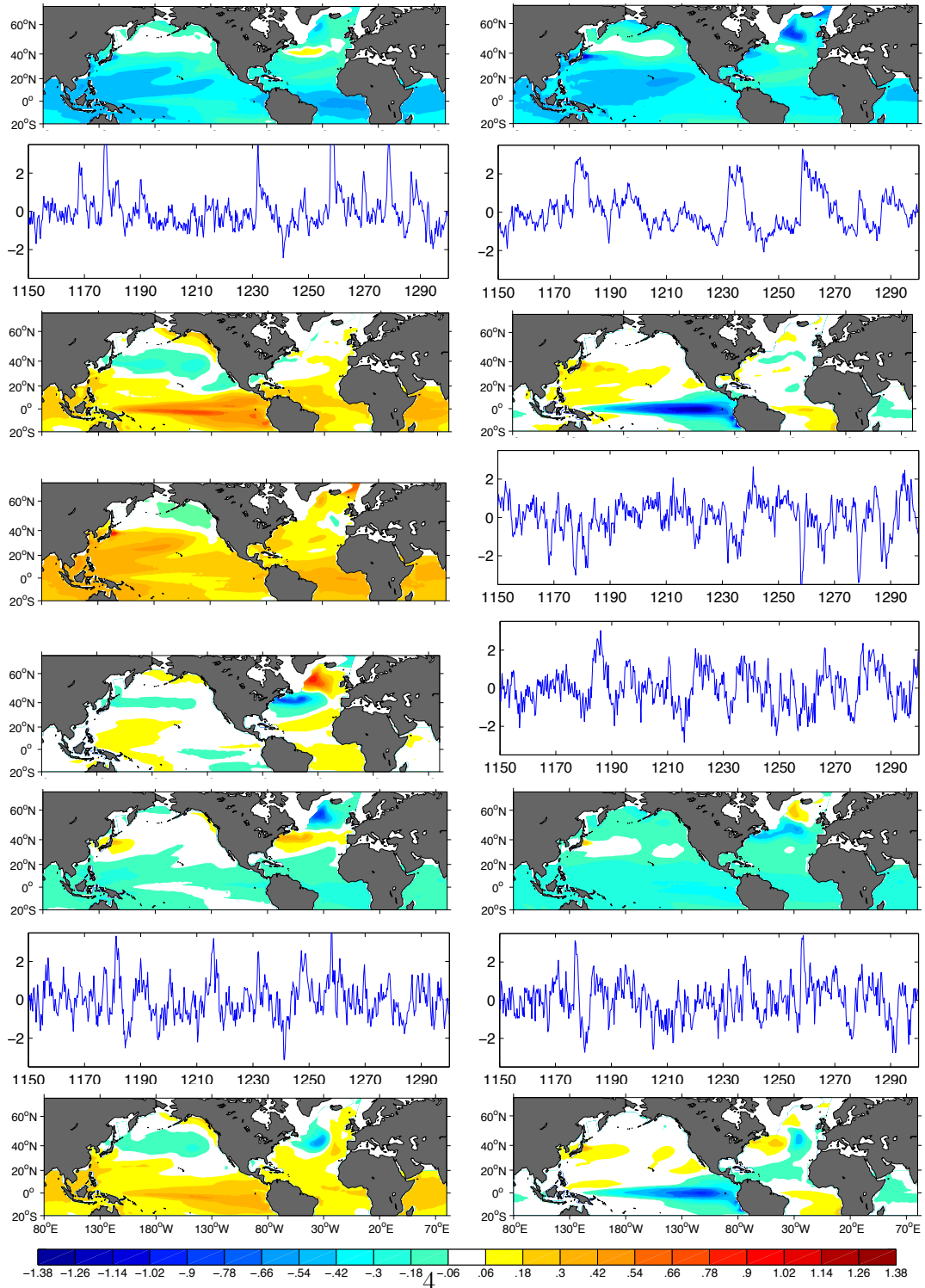
Figure 5.8: Normal modes (in °C) of the deterministic matrix B . Mode 1/2 (1st row), and its associated time series (2nd row), 3/4 (3rd row), 5 and its associated time series (4th row), 6 and its associated time series (5th row), 7/8 (6th row), 9/10 (bottom). LIM made from MILL (1150-1300).
