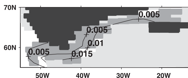
FIG. 14. Regression of low-pass-filtered ( T_c = 10 yr) salinity anomalies on the isopycnal surface 27\sigma_\theta onto the SAM index, when the latter leads by 65 yr. Contour interval is 0.005 psu. The gray shaded areas indicate that the regression is 10% significant. The light shading indicates grid points where the regression is not computed, as the density of 27\sigma_\theta is reached less than 60% of the year.
