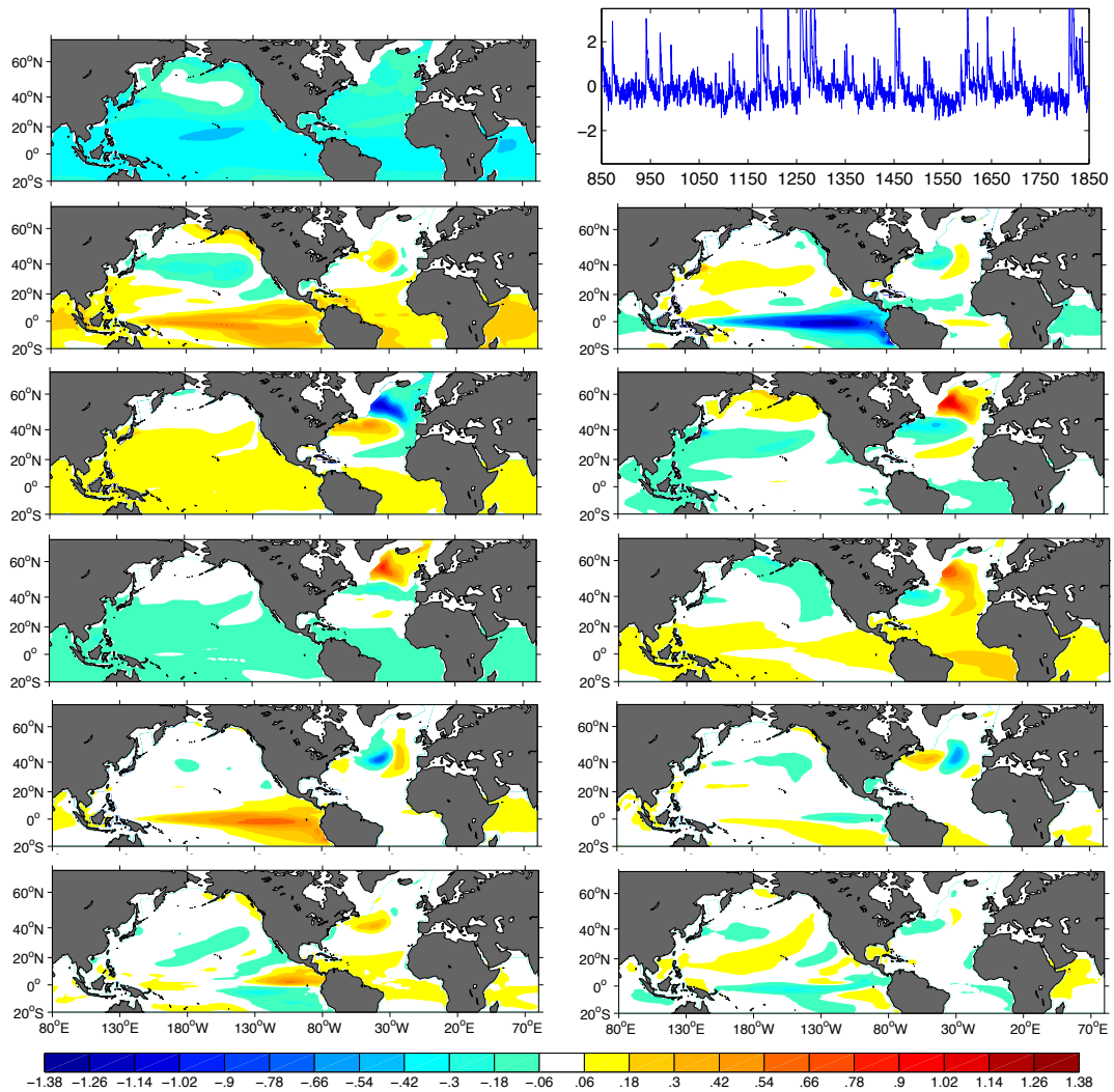
Figure 5.6: Normal modes (in ^{\circ}\text{C} ) of the deterministic matrix \mathbf{B} . Mode 1 and its associated time series (1st row), 2/3 (2nd row), 4/5 (3rd row), 6/7 (4th row), 8/9 (5th row), and 11/12 (bottom). LIM made from MILL (850-1849).
