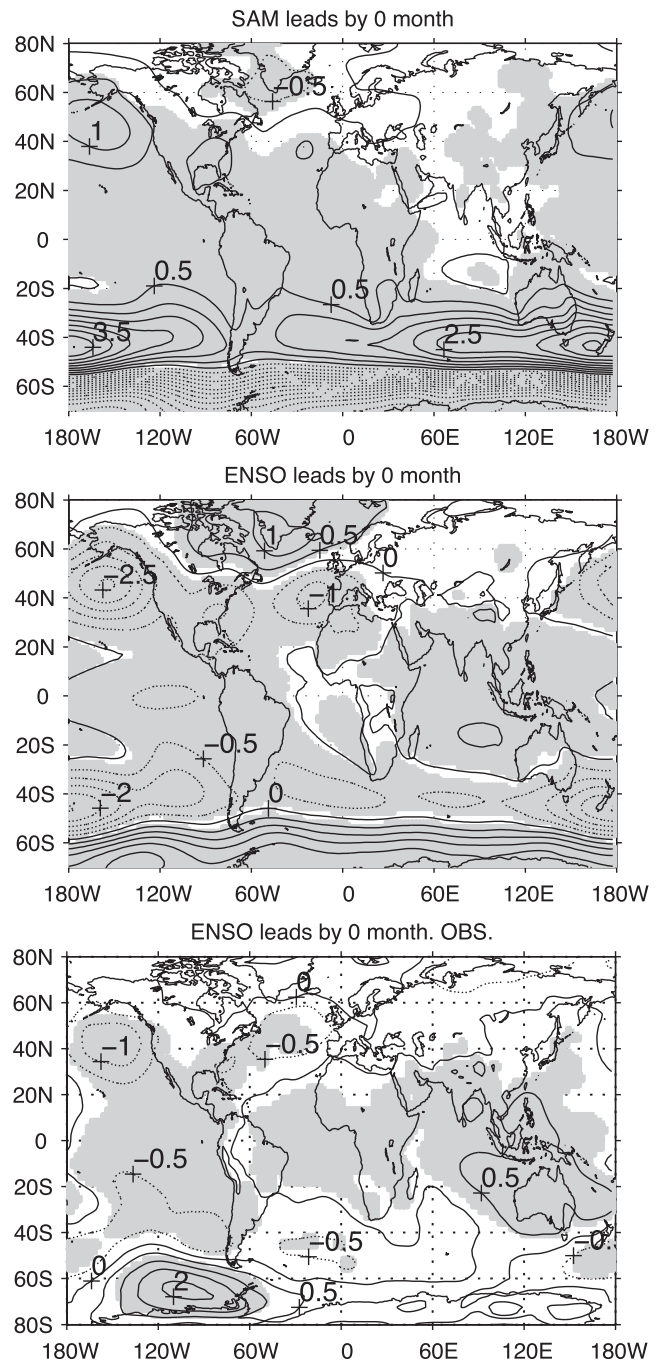
FIG. 8. Regression of monthly anomalies of the SLP mapped onto (top) the SAM index in the model, (middle) ENSO in the model, and (bottom) ENSO in the observations during 1993–2008. Contour interval is 0.5 hPa. Dashed lines correspond to negative values. The shaded areas indicate that the regression is 5% significant.
