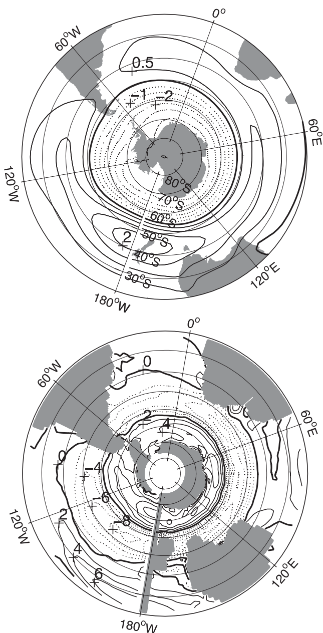
FIG. 4. (top) The SAM pattern, represented by the first EOF of the yearly SLP anomalies south of 20^{\circ}\text{S} . The EOF time series (SAM index) is normalized, and the contour interval is 0.5\text{ hPa} . (bottom) Regression of annual anomalies of Ekman pumping on the SAM index. Contour interval is 2\text{ m yr}^{-1} . Dashed lines correspond to negative values and the thick lines to zero.
