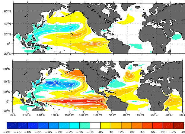
Figure 4.19: Optimal initial structure (top) leading to maximum amplification (bottom) of SST variance in the Tropical Strip. LIM made from IPSLCM5 (control).
