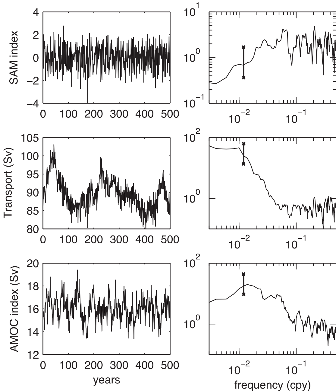
FIG. 3. (left) Time series and (right) power spectrum of, from top to bottom, the SAM index, the mass transport across the Drake Passage (in Sv), and the AMOC maximum below 500 m and between 30° and 60°N (in Sv). Power spectra are estimated with the multitaper method (seven tapers). The 95% confidence interval is indicated.
