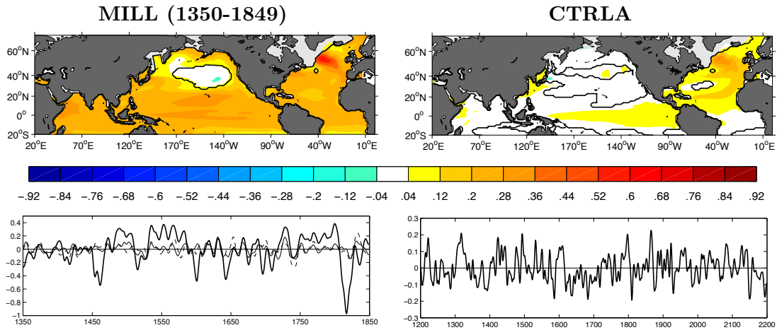
Figure 5.9: Top : SSTs (in °C) associated with the traditional AMO in MILL (1350-1849) (left) and in CTRLA (right). Bottom left: Traditional AMO (in °C, thick line), AMO-Vol (solid line) and AMO-Vol/EN (dashed line) in MILL (1350-1849). Bottom right : Traditional AMO in CTRLA; note the change of scale. The black contour indicates 5% significance.
