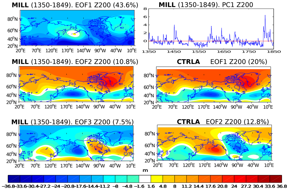
Figure 5.18: EOFs of annual geopotential heights anomalies at 200 mB in MILL (1350-1849) and in CTRLA. The percentage indicates the explained variance by each EOF.
