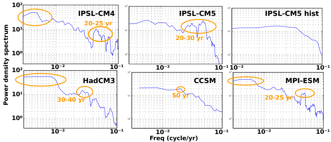
Figure 4.4: Power density spectrum of the first principal component of low-pass filtered ( T_c = 10 yr) AMOC anomalies in IPSL-CM4 (top left), IPSL-CM5 (top middle), historical IPSL-CM5 simulation (top right), HadCM3 (bottom left), CCSM (bottom middle), and MPI (bottom right).
