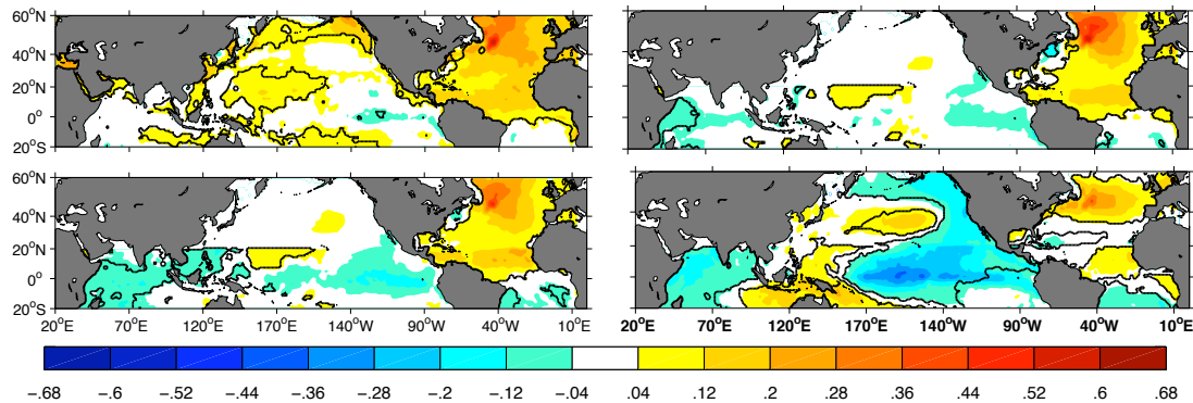
Figure 4.27: SST pattern (in ^{\circ}\text{C} ) associated with the AMO time series in Fig.4.26. Top left : traditional AMO, Top right : AMO-GT, Bottom left : AMO-GT/EN, Bottom right : AMO-GT/EN/PD. LIM made from observed SST. The black contour indicates 5% significance.
