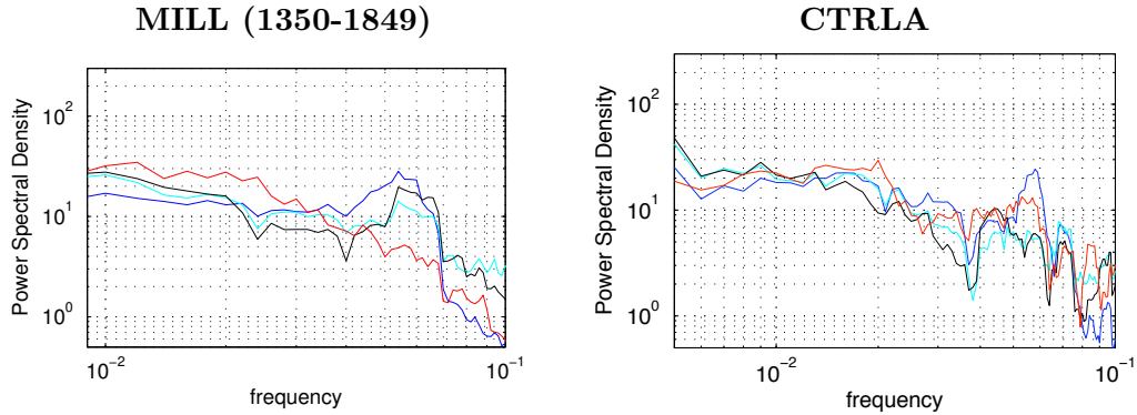
Figure 5.12: Power spectral density of low-pass filtered AMOC maximum between 10 and 60° N (blue), AMOC maximum at 30° N (cyan), AMOC-PC1 (black), and AMO (red) in MILL (1350-1849) (left) and in CTRLA (right).
