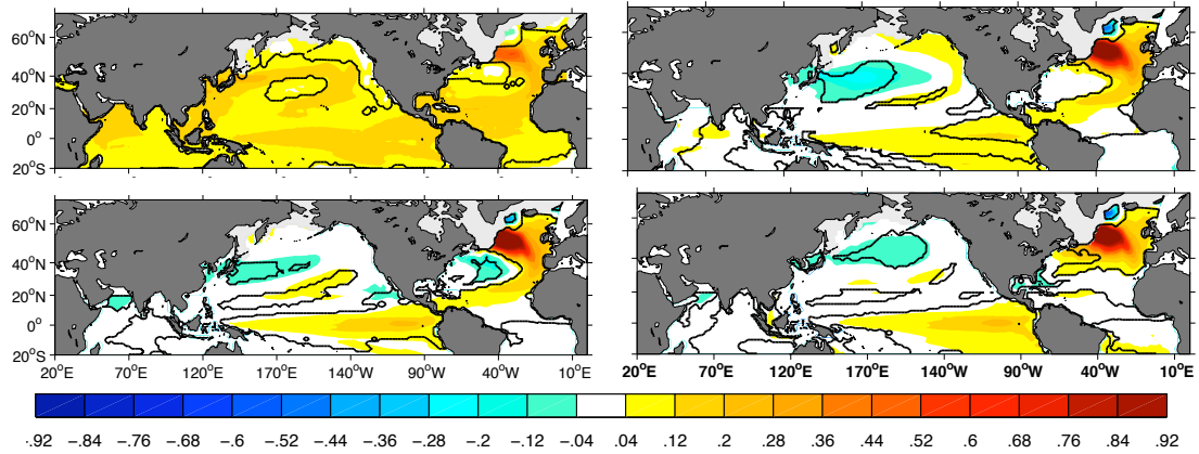
Figure 4.11: SST pattern (in °C) associated with the AMO time series in Fig.4.10. Top left : traditional AMO, Top right : AMO-GT, Bottom left : AMO-GT/EN, Bottom right : AMO-GT/EN/PD. LIM made from the historical IPSLCM5 simulation. The black contour indicates 5% significance.
