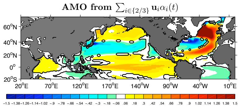
Figure 5.19: SSTs (in °C) associated with the AMO computed from \sum_{i \in \{2/3\}} \mathbf{u}_i \alpha_i(t) . The black contour indicates 5% significance. LIM made from MILL (1350-1849)
