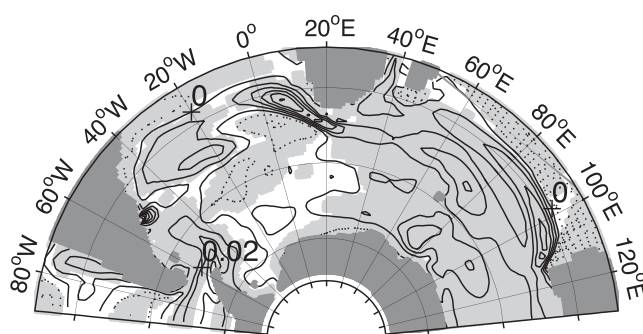
FIG. 5. Regression of annual anomalies of the averaged salinity between 0 and 100 m onto the SAM index when the SAM leads by 1 yr. Contour interval is 0.01\text{ psu} ; dashed lines correspond to negative values. The shaded areas indicate that the regression is 5% significant.
