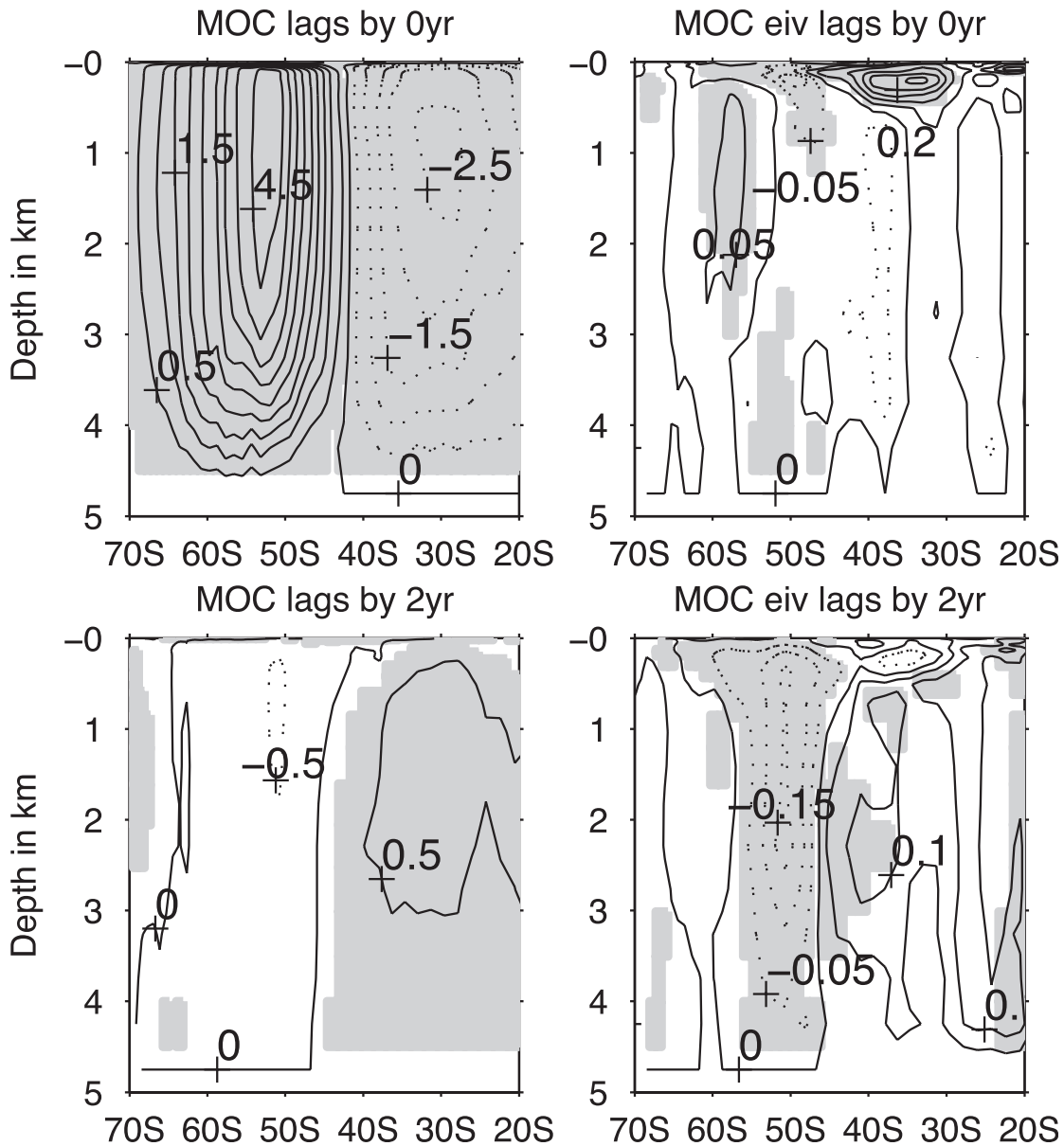
FIG. 6. (left) Regression of annual anomalies of the global MOC and (right) the eddy contribution to it on the SAM index at (top) zero lag and (bottom) 2 yr after. Contour interval is (left) 0.5 Sv and (right) 0.05 Sv. Dashed lines correspond to negative values. The shaded areas indicate that the regression is 5% significant.
