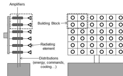
Figure 3-7. Active antenna description (adapted from(Roger 1999))
