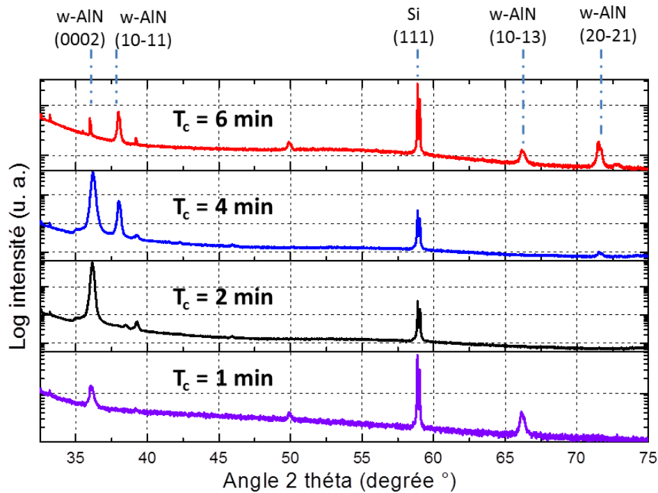
Figure 3.26 : spectres XRD des échantillons AlN-Si-06, AlN-Si-08, AlN-Si-09 et AlN-Si-11.
