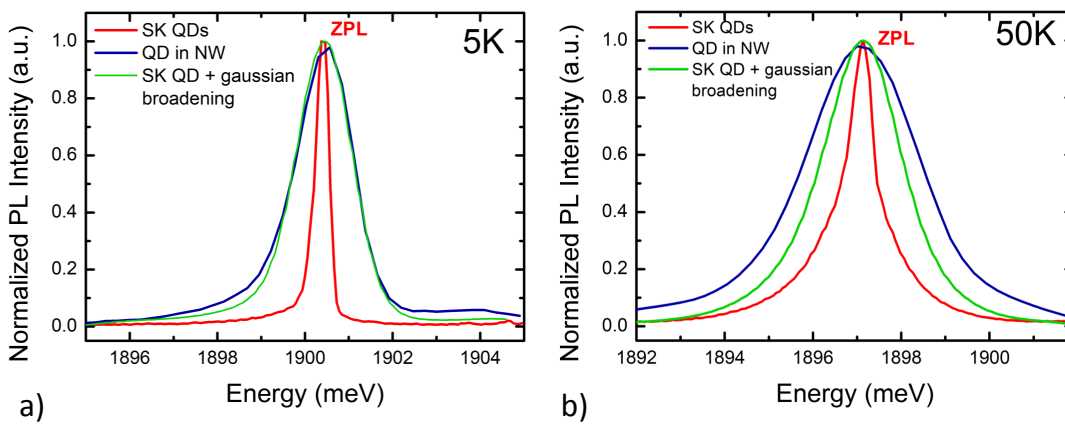
FIGURE 3.36: a) Photoluminescence spectra of the single CdTe/ZnTe self-assembled QD (red line) and NW QD (blue line) recorded at 5 K. The green line corresponds to the convolution of the PL spectra with Gaussian line. b) 50 K photoluminescence spectra of the same objects.
