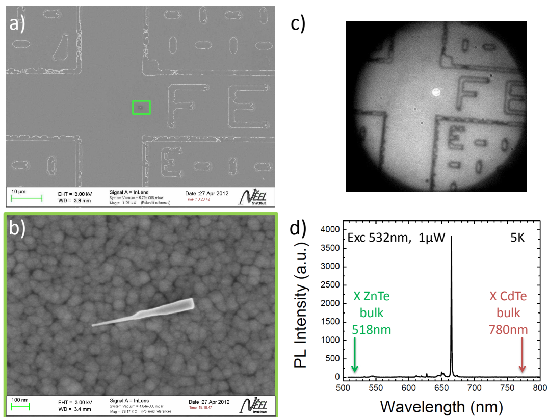
FIGURE 3.14: a) High-resolution SEM image of patterned silicon substrate. b) High-resolution SEM image of studied nanowire. c) Image obtained with optic microscope with superposed image of nanowire luminescence (white spot). d) Micro-photoluminescence spectra of the studied nanowire.
