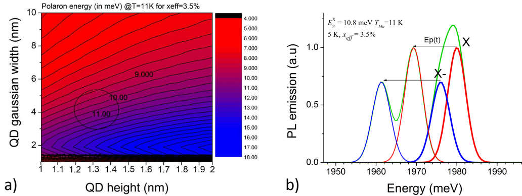
FIGURE 2.34: a) Exciton magnetic polaron energy plotted as a function of lateral size and height of the quantum dot. b) Calculated spectrum of a single CdMn(8.3%)Te quantum dot before (bold solid lines) and after (thin lines) the MP formation
