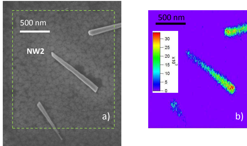
FIGURE 3.7: a) High resolution SEM image of 3 broken ZnTe NWs deposited on a silicon substrate. b) CL image of the NWs shown in (a) recorded at 5 K.
