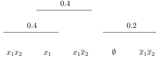
Figure 6.2: An example of induced observations
