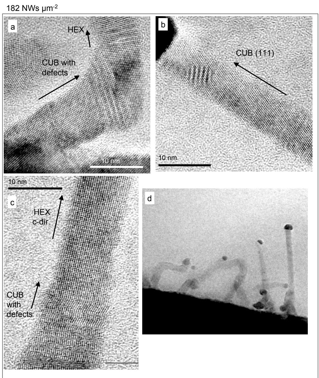
Figure 4.5: HRTEM images of ZnSe nanowires grown in identical conditions except for varying surface densities. (a)-(c) Images showing typical crystal structure characteristics found in a sample with \sigma_{NW} = 182 \text{ NW } \mu\text{m}^{-2} ; (d) TEM view of an ensemble of nanowires from this sample.
