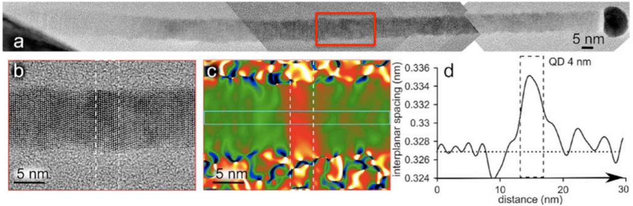
Figure 6.5: Structural analysis by TEM of single ZnSe/CdSe NW-QD. (a) Series of HRTEM images along and entire tilted NW attached to the substrate. The CdSe QD is located in the boxed region about 70 nm from the gold catalyst particle. (b) HRTEM of the boxed region in panel (a): the dashed rectangle in panels (b) to (d) corresponds to the CdSe slice. (c) Geometrical phase analysis of the growth planes along the growth direction. (d) Line profile extracted from the solid boxed region drawn in panel (c). The (0002) interplanar spacing for ZnSe is indicated by the horizontal dashed line. Taken from ref. [51].
