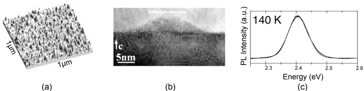
Figure 1.10: (a) AFM image of QD ensemble on substrate; density 10^{10} \text{ cm}^{-2} . (b) HRTEM image of CdSe self-assembled (SK) QD. 2D to 3D transition obtained with a treatment under amorphous Se; with amorphous Se capping layer (from [38]). (c) Photoluminescence of QD ensemble. Modified from Ref. [23].
